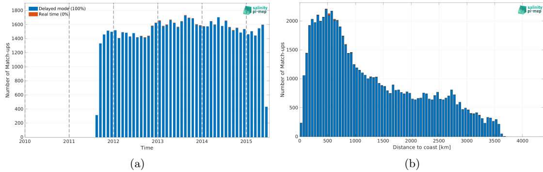
Figure 2: Number of match-ups between Argo and Aquarius SSS L3 OR v5 - 7-Day running - Rain mask (NASA-GSFC) SSS as a function of time (a) and as function of the distance to coast (b) over the South Pacific Ocean Pi-MEP region and for the full satellite product period.
