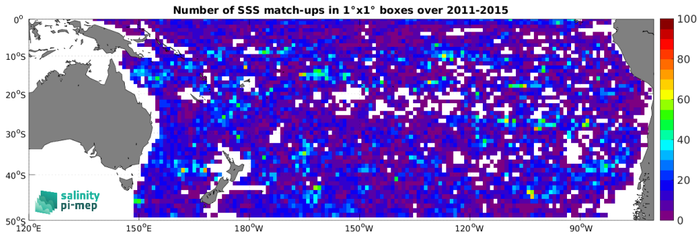
Figure 5: Number of SSS match-ups between Argo SSS and the Aquarius SSS L3 OR v5 - 7-Day running - Rain mask (NASA-GSFC) SSS product for the South Pacific Ocean Pi-MEP region over 1^\circ \times 1^\circ boxes and for the full satellite product period.
