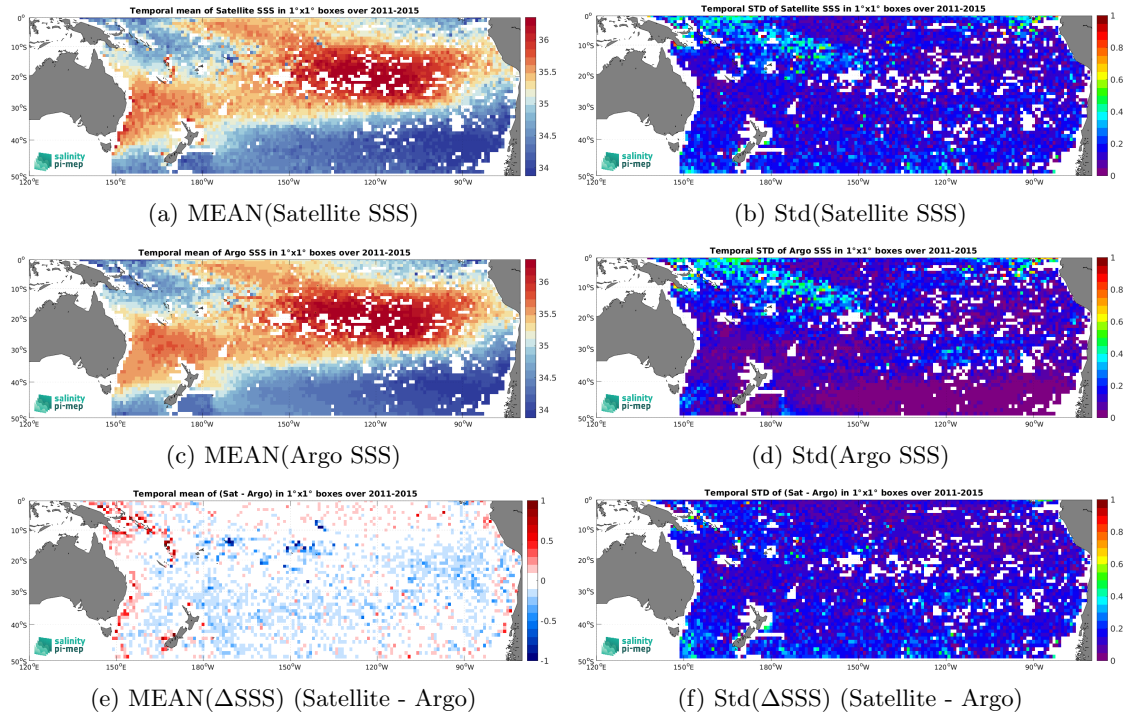
Figure 7: Temporal mean (left) and Std (right) of SSS from Aquarius SSS L3 OR v5 - 7-Day running - Rain mask (NASA-GSFC) (top), Argo (middle), and of \Delta SSS (Satellite - Argo). Only match-up pairs are used to generate these maps.
