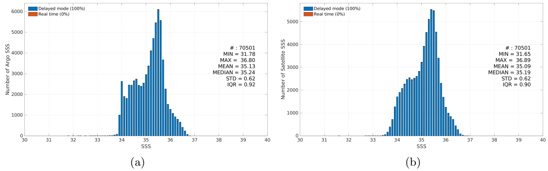
Figure 3: Histograms of SSS from Argo (a) and Aquarius SSS L3 OR v5 - 7-Day running - Rain mask (NASA-GSFC) (b) considering all match-up pairs per bins of 0.1 over the South Pacific Ocean Pi-MEP region and for the full satellite product period.
