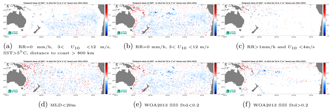
Figure 14: Temporal mean gridded over spatial boxes of size 1^\circ \times 1^\circ of \Delta\text{SSS} (Aquarius SSS L3 OR v5 - 7-Day running - Rain mask (NASA-GSFC) - Argo) for 6 different subdatasets corresponding to: RR=0 mm/h, 3 < U_{10} < 12 m/s, SST > 5°C, distance to coast > 800 km (a), RR=0 mm/h, 3 < U_{10} < 12 m/s (b), RR > 1mm/h and U_{10} < 4 m/s (c), MLD < 20m (d), WOA2013 SSS Std < 0.2 (e), WOA2013 SSS Std > 0.2 (f).
