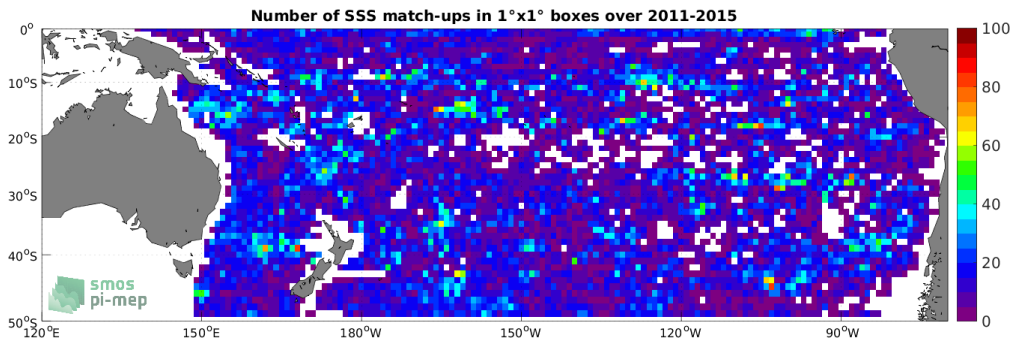
Figure 4: Number of SSS match-ups between Argo SSS and the Aquarius SSS L3 OR v5 - 7-Day running - Rain mask (NASA-GSFC) SSS product for the South Pacific Ocean Pi-MEP region over 1^{\circ} \times 1^{\circ} boxes and for the full satellite product period.
