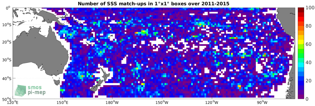
Figure 4: Number of SSS match-ups between Argo SSS and the Aquarius SSS L3 OR v5 - 7-Day running - Rain mask (NASA-GSFC) SSS product for the South Pacific Ocean Pi-MEP region over 1^\circ \times 1^\circ boxes and for the full satellite product period.
