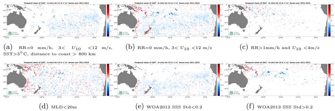
Figure 12: Temporal mean gridded over spatial boxes of size 1^\circ \times 1^\circ of \Delta SSS (Aquarius SSS L3 OR v5 - 7-Day running - Rain mask (NASA-GSFC) - Argo) for 6 different subdatasets corresponding to:RR=0 mm/h, 3 < U_{10} < 12 m/s, SST >5^\circ C, distance to coast > 800 km (a), RR=0 mm/h, 3 < U_{10} < 12 m/s (b), RR >1 mm/h and U_{10} < 4 m/s (c),MLD <20 m (d),WOA2013 SSS Std <0.2 (e),WOA2013 SSS Std >0.2 (f).
