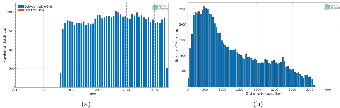
Figure 1: Number of match-ups between Argo and Aquarius SSS L3 OR v5 - 7-Day running - Rain mask (NASA-GSFC) SSS as a function of time (a) and as function of the distance to coast (b) over the South Pacific Ocean Pi-MEP region and for the full satellite product period.
