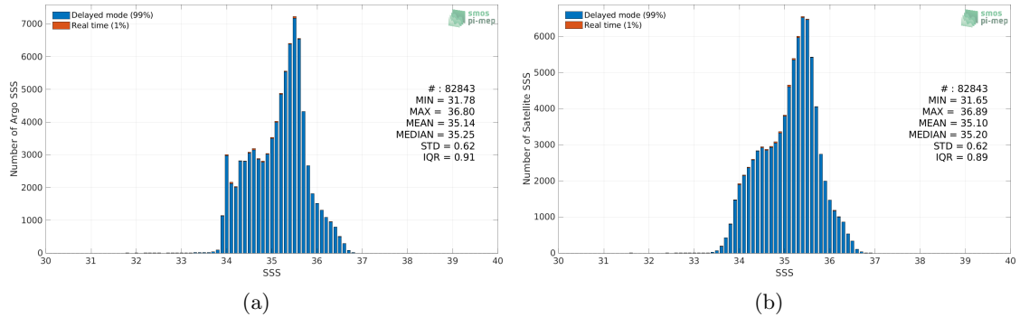
Figure 2: Histograms of SSS from Argo (a) and Aquarius SSS L3 OR v5 - 7-Day running - Rain mask (NASA-GSFC) (b) considering all match-up pairs per bins of 0.1 over the South Pacific Ocean Pi-MEP region and for the full satellite product period.
