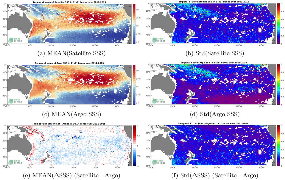
Figure 6: Temporal mean (left) and Std (right) of SSS from Aquarius SSS L3 OR v5 - 7-Day running - Rain mask (NASA-GSFC) (top), Argo (middle), and of \Delta SSS (Satellite - Argo). Only match-up pairs are used to generate these maps.
