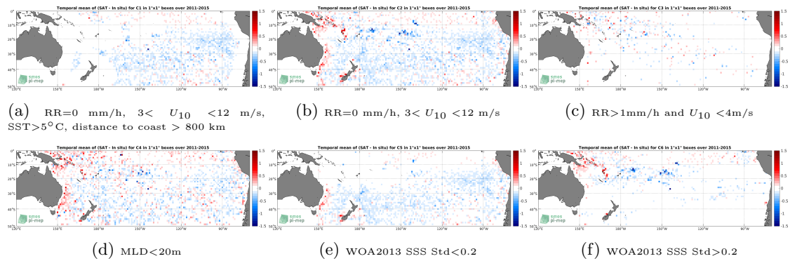
Figure 12: Temporal mean gridded over spatial boxes of size 1^\circ \times 1^\circ of \Delta SSS (Aquarius-L3-OR-V5-7DAY-RUNNING-RAIN-MASK-1DEG - Argo) for 6 different subdatasets corresponding to:RR=0 mm/h, 3 < U_{10} < 12 m/s, SST >5^\circ C, distance to coast > 800 km (a), RR=0 mm/h, 3 < U_{10} < 12 m/s (b), RR >1 mm/h and U_{10} < 4 m/s (c),MLD <20 m (d),WOA2013 SSS Std <0.2 (e),WOA2013 SSS Std >0.2 (f).
