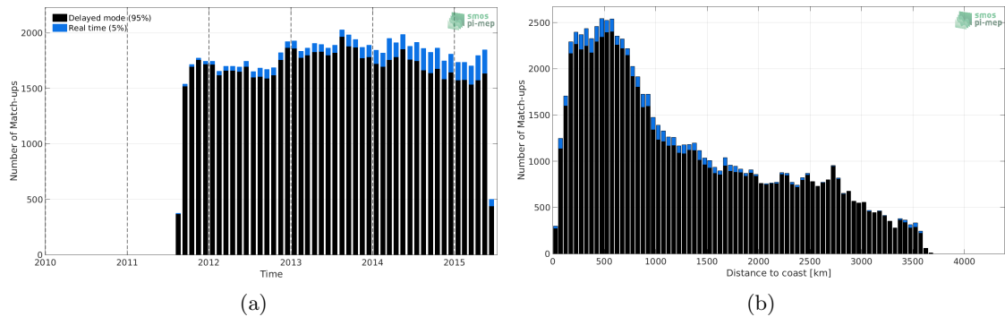
Figure 1: Number of match-ups between Argo and Aquarius-L3-OR-V5-7DAY-RUNNING-RAIN-MASK-1DEG SSS as a function of time (a) and as function of the distance to coast (b) over the South Pacific Ocean Pi-MEP region and for the full satellite product period.
