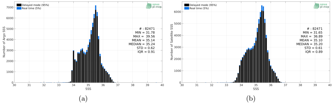
Figure 2: Histograms of SSS from Argo (a) and Aquarius-L3-OR-V5-7DAY-RUNNING-RAIN-MASK-1DEG (b) considering all match-up pairs per bins of 0.1 over the South Pacific Ocean Pi-MEP region and for the full satellite product period.
