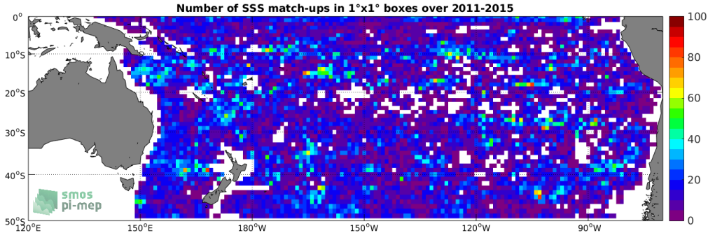
Figure 4: Number of SSS match-ups between Argo SSS and the Aquarius-L3-OR-V5-7DAY-RUNNING-RAIN-MASK-1DEG SSS product for the South Pacific Ocean Pi-MEP region over 1^\circ \times 1^\circ boxes and for the full satellite product period.
