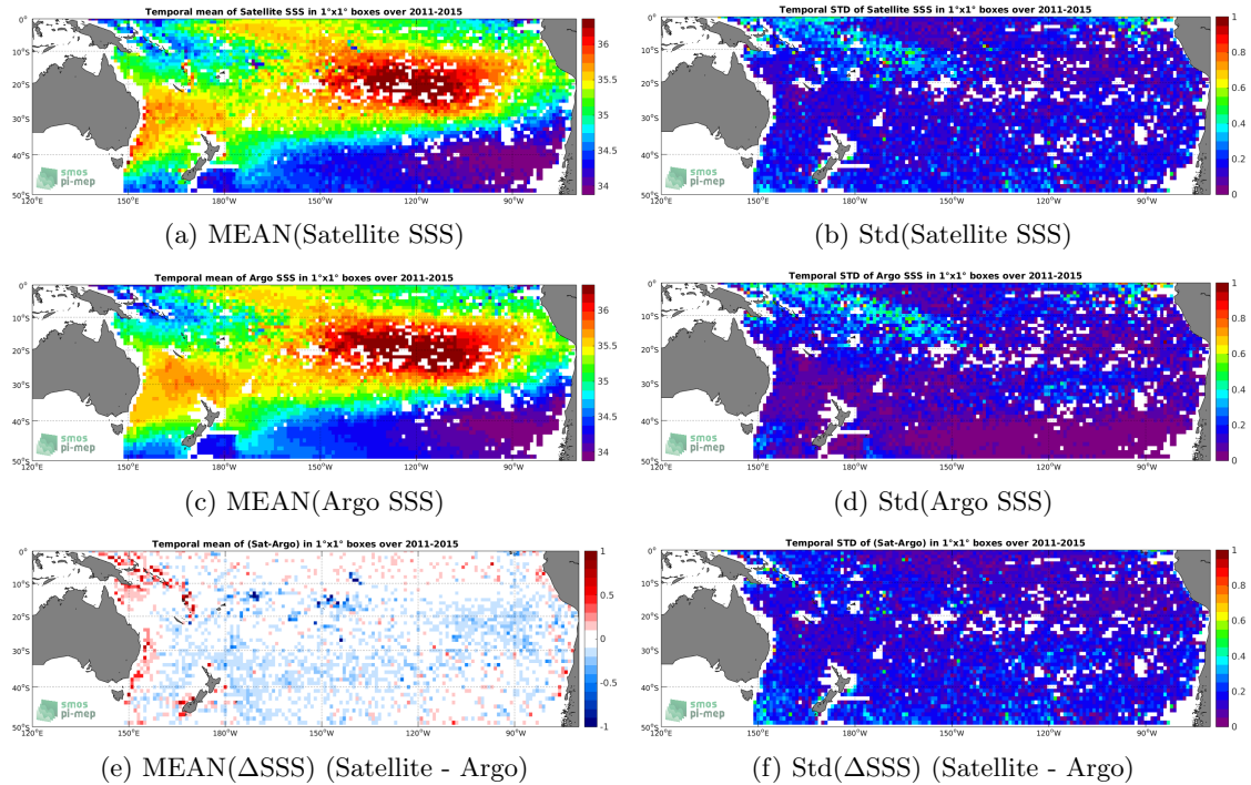
Figure 6: Temporal mean (left) and Std (right) of SSS from Aquarius-L3-OR-V5-7DAY-RUNNING-RAIN-MASK-1DEG (top), Argo (middle), and of \Delta SSS (Satellite - Argo). Only match-up pairs are used to generate these maps.
