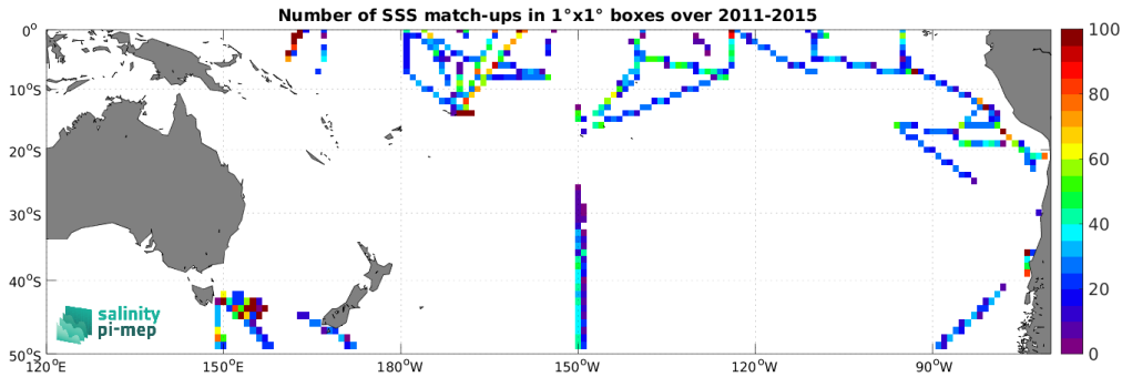
Figure 5: Number of SSS match-ups between TSG (SAMOS) SSS and the Aquarius SSS L3 OR v5 - Monthly (NASA-GSFC) SSS product for the South Pacific Ocean Pi-MEP region over 1^\circ \times 1^\circ boxes and for the full satellite product period.
