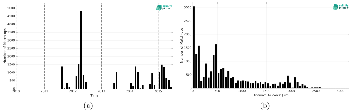
Figure 2: Number of match-ups between TSG (SAMOS) and Aquarius SSS L3 OR v5 - Monthly (NASA-GSFC) SSS as a function of time (a) and as function of the distance to coast (b) over the South Pacific Ocean Pi-MEP region and for the full satellite product period.
