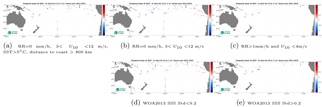
Figure 14: Temporal mean gridded over spatial boxes of size 1^\circ \times 1^\circ of \Delta\text{SSS} (Aquarius SSS L3 OR v5 - Monthly (NASA-GSFC) - TSG (SAMOS)) for 5 different subdatasets corresponding to:RR=0 mm/h, 3 < U_{10} < 12 m/s, SST>5°C, distance to coast > 800 km (a), RR=0 mm/h, 3 < U_{10} < 12 m/s (b), RR>1mm/h and U_{10} < 4 m/s (c), WOA2013 SSS Std<0.2 (d), WOA2013 SSS Std>0.2 (e).
