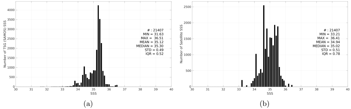
Figure 3: Histograms of SSS from TSG (SAMOS) (a) and Aquarius SSS L3 OR v5 - Monthly (NASA-GSFC) (b) considering all match-up pairs per bins of 0.1 over the South Pacific Ocean Pi-MEP region and for the full satellite product period.
