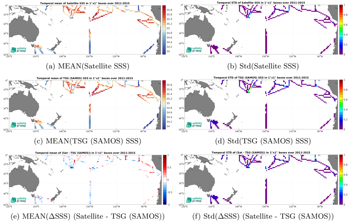
Figure 7: Temporal mean (left) and Std (right) of SSS from Aquarius SSS L3 OR v5 - Monthly (NASA-GSFC) (top), TSG (SAMOS) (middle), and of \Delta SSS (Satellite - TSG (SAMOS)). Only match-up pairs are used to generate these maps.
