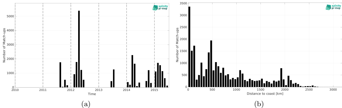
Figure 1: Number of match-ups between TSG (SAMOS) and Aquarius SSS L3 OR v5 - Monthly (NASA-GSFC) SSS as a function of time (a) and as function of the distance to coast (b) over the South Pacific Ocean Pi-MEP region and for the full satellite product period.
