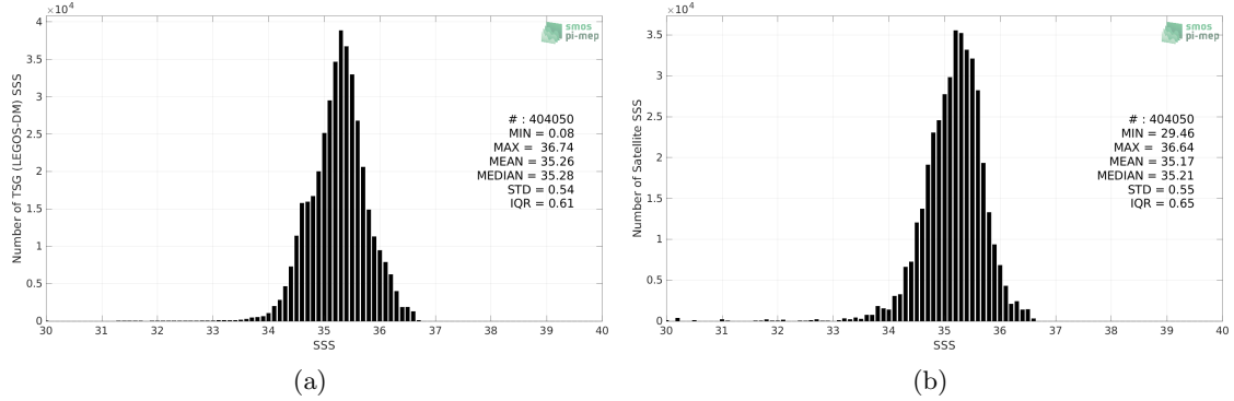
Figure 2: Histograms of SSS from TSG (LEGOS-DM) (a) and Aquarius SSS L3 OR v5 - Monthly (NASA-GSFC) (b) considering all match-up pairs per bins of 0.1 over the South Pacific Ocean Pi-MEP region and for the full satellite product period.
