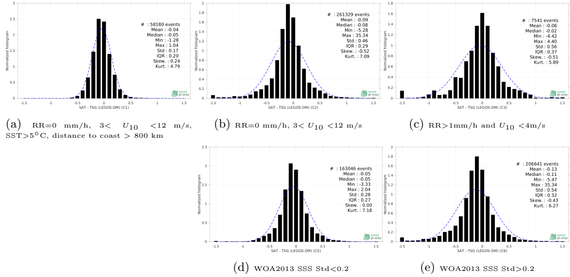
Figure 13: Normalized histogram of \Delta SSS (Aquarius SSS L3 OR v5 - Monthly (NASA-GSFC) - TSG (LEGOS-DM)) for 5 different subdatasets corresponding to: RR=0 mm/h, 3 < U_{10} < 12 m/s, SST > 5°C, distance to coast > 800 km (a), RR=0 mm/h, 3 < U_{10} < 12 m/s (b), RR > 1mm/h and U_{10} < 4 m/s (c), WOA2013 SSS Std < 0.2 (d), WOA2013 SSS Std > 0.2 (e).
