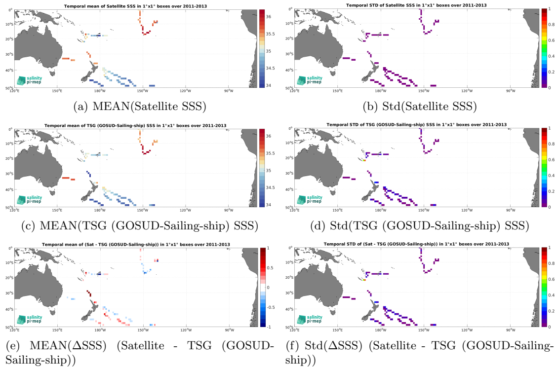
Figure 7: Temporal mean (left) and Std (right) of SSS from Aquarius SSS L3 OR v5 - Monthly (NASA-GSFC) (top), TSG (GOSUD-Sailing-ship) (middle), and of \Delta SSS (Satellite - TSG (GOSUD-Sailing-ship)). Only match-up pairs are used to generate these maps.
