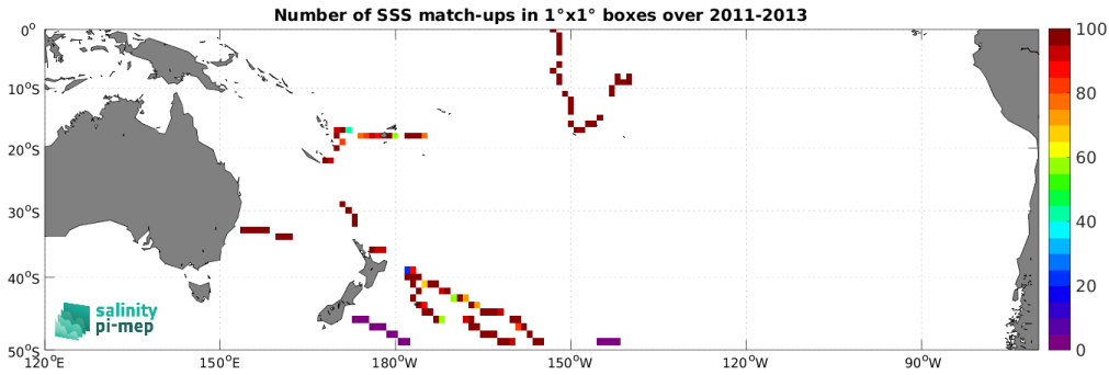
Figure 5: Number of SSS match-ups between TSG (GOSUD-Sailing-ship) SSS and the Aquarius SSS L3 OR v5 - Monthly (NASA-GSFC) SSS product for the South Pacific Ocean Pi-MEP region over 1^\circ \times 1^\circ boxes and for the full satellite product period.
