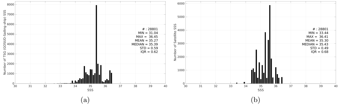
Figure 3: Histograms of SSS from TSG (GOSUD-Sailing-ship) (a) and Aquarius SSS L3 OR v5 - Monthly (NASA-GSFC) (b) considering all match-up pairs per bins of 0.1 over the South Pacific Ocean Pi-MEP region and for the full satellite product period.
