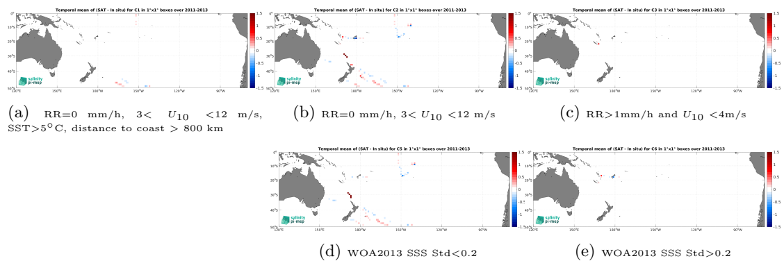
Figure 14: Temporal mean gridded over spatial boxes of size 1^\circ \times 1^\circ of \Delta SSS (Aquarius SSS L3 OR v5 - Monthly (NASA-GSFC) - TSG (GOSUD-Sailing-ship)) for 5 different subdatasets corresponding to:RR=0 mm/h, 3 < U_{10} < 12 m/s, SST >5^\circ\text{C} , distance to coast > 800 km (a), RR=0 mm/h, 3 < U_{10} < 12 m/s (b), RR >1 mm/h and U_{10} < 4 m/s (c), WOA2013 SSS Std <0.2 (d), WOA2013 SSS Std >0.2 (e).
