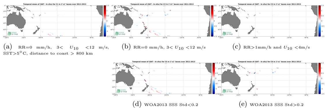
Figure 12: Temporal mean gridded over spatial boxes of size 1^\circ \times 1^\circ of \Delta SSS (Aquarius-L3-OR-V5-MONTHLY-1DEG - TSG-GOSUD-Sailing-ship) for 5 different subdatasets corresponding to:RR=0 mm/h, 3 < U_{10} < 12 m/s, SST>5°C, distance to coast > 800 km (a), RR=0 mm/h, 3 < U_{10} < 12 m/s (b), RR>1mm/h and U_{10} < 4 m/s (c), WOA2013 SSS Std<0.2 (d), WOA2013 SSS Std>0.2 (e).
