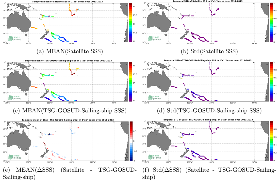
Figure 6: Temporal mean (left) and Std (right) of SSS from Aquarius-L3-OR-V5-MONTHLY-1DEG (top), TSG-GOSUD-Sailing-ship (middle), and of \Delta SSS (Satellite - TSG-GOSUD-Sailing-ship). Only match-up pairs are used to generate these maps.
