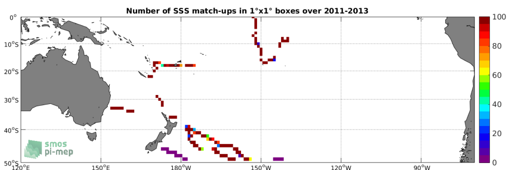
Figure 4: Number of SSS match-ups between TSG-GOSUD-Sailing-ship SSS and the Aquarius-L3-OR-V5-MONTHLY-1DEG SSS product for the South Pacific Ocean Pi-MEP region over 1^\circ \times 1^\circ boxes and for the full satellite product period.
