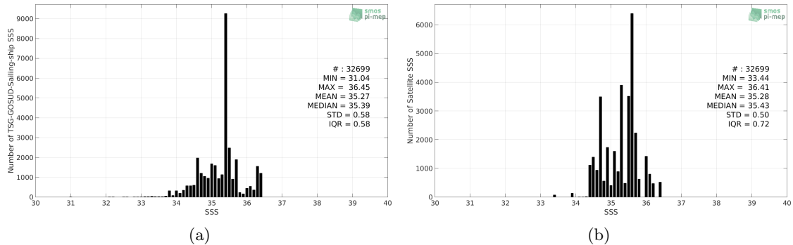
Figure 2: Histograms of SSS from TSG-GOSUD-Sailing-ship (a) and Aquarius-L3-OR-V5-MONTHLY-1DEG (b) considering all match-up pairs per bins of 0.1 over the South Pacific Ocean Pi-MEP region and for the full satellite product period.
