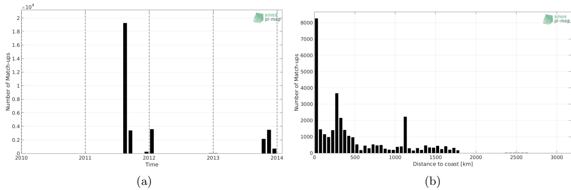
Figure 1: Number of match-ups between TSG-GOSUD-Sailing-ship and Aquarius-L3-OR-V5-MONTHLY-1DEG SSS as a function of time (a) and as function of the distance to coast (b) over the South Pacific Ocean Pi-MEP region and for the full satellite product period.
