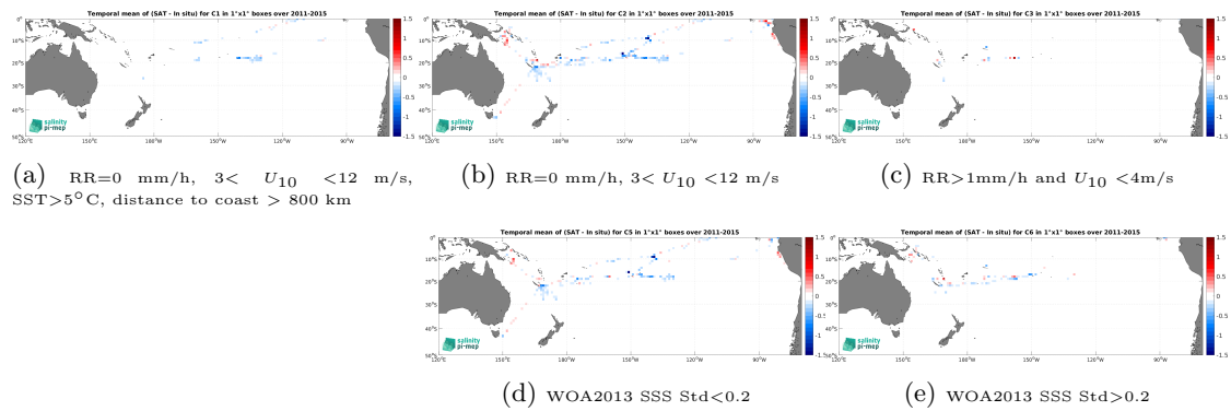
Figure 14: Temporal mean gridded over spatial boxes of size 1^\circ \times 1^\circ of \Delta SSS (Aquarius SSS L3 OR v5 - Monthly (NASA-GSFC) - TSG (GOSUD-Research-vessel)) for 5 different subdatasets corresponding to:RR=0 mm/h, 3 < U_{10} < 12 m/s, SST >5^\circ\text{C} , distance to coast > 800 km (a), RR=0 mm/h, 3 < U_{10} < 12 m/s (b), RR >1 mm/h and U_{10} < 4 m/s (c), WOA2013 SSS Std <0.2 (d), WOA2013 SSS Std >0.2 (e).
