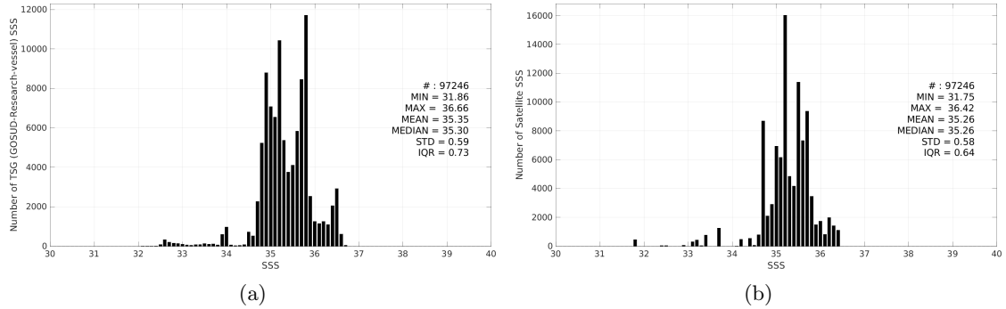
Figure 3: Histograms of SSS from TSG (GOSUD-Research-vessel) (a) and Aquarius SSS L3 OR v5 - Monthly (NASA-GSFC) (b) considering all match-up pairs per bins of 0.1 over the South Pacific Ocean Pi-MEP region and for the full satellite product period.
