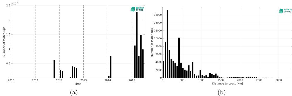
Figure 2: Number of match-ups between TSG (GOSUD-Research-vessel) and Aquarius SSS L3 OR v5 - Monthly (NASA-GSFC) SSS as a function of time (a) and as function of the distance to coast (b) over the South Pacific Ocean Pi-MEP region and for the full satellite product period.
