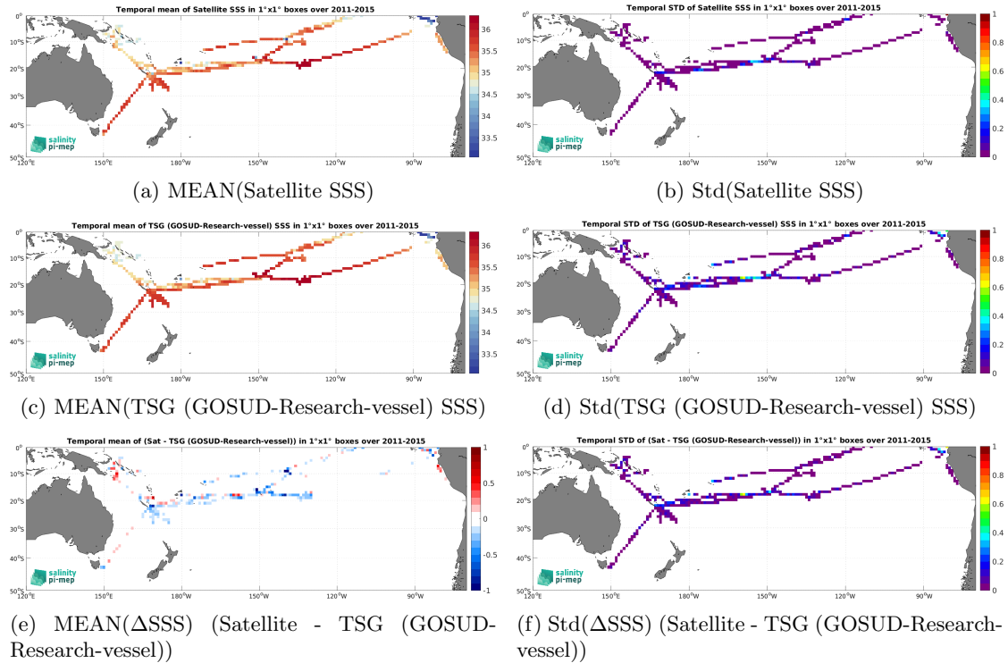
Figure 7: Temporal mean (left) and Std (right) of SSS from Aquarius SSS L3 OR v5 - Monthly (NASA-GSFC) (top), TSG (GOSUD-Research-vessel) (middle), and of \Delta SSS (Satellite - TSG (GOSUD-Research-vessel)). Only match-up pairs are used to generate these maps.
