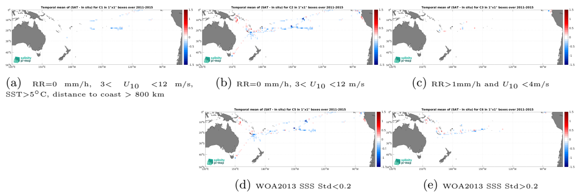
Figure 12: Temporal mean gridded over spatial boxes of size 1^\circ \times 1^\circ of \Delta\text{SSS} (Aquarius SSS L3 OR v5 - Monthly (NASA-GSFC) - TSG (GOSUD-Research-vessel)) for 5 different subdatasets corresponding to:RR=0 mm/h, 3 < U_{10} < 12 m/s, SST >5^\circ\text{C} , distance to coast > 800 km (a), RR=0 mm/h, 3 < U_{10} < 12 m/s (b), RR >1 mm/h and U_{10} < 4 m/s (c), WOA2013 SSS Std <0.2 (d), WOA2013 SSS Std >0.2 (e).
