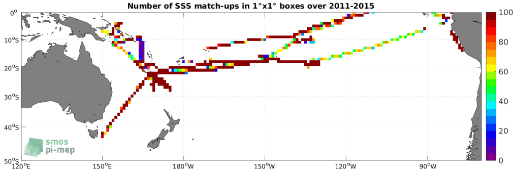
Figure 4: Number of SSS match-ups between TSG (GOSUD-Research-vessel) SSS and the Aquarius SSS L3 OR v5 - Monthly (NASA-GSFC) SSS product for the South Pacific Ocean Pi-MEP region over 1^\circ \times 1^\circ boxes and for the full satellite product period.
