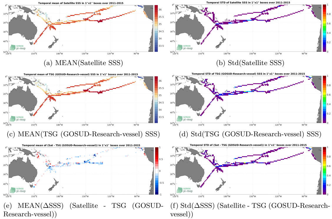
Figure 6: Temporal mean (left) and Std (right) of SSS from Aquarius SSS L3 OR v5 - Monthly (NASA-GSFC) (top), TSG (GOSUD-Research-vessel) (middle), and of \Delta SSS (Satellite - TSG (GOSUD-Research-vessel)). Only match-up pairs are used to generate these maps.
