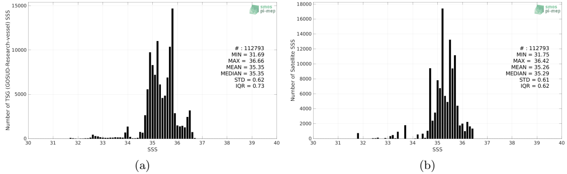
Figure 2: Histograms of SSS from TSG (GOSUD-Research-vessel) (a) and Aquarius SSS L3 OR v5 - Monthly (NASA-GSFC) (b) considering all match-up pairs per bins of 0.1 over the South Pacific Ocean Pi-MEP region and for the full satellite product period.
