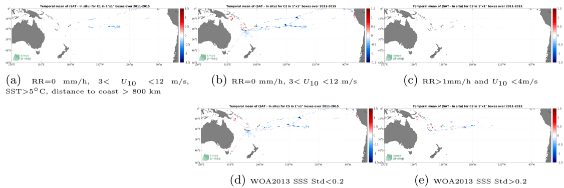
Figure 12: Temporal mean gridded over spatial boxes of size 1^\circ \times 1^\circ of \Delta SSS (Aquarius SSS L3 OR v5 - Monthly (NASA-GSFC) - TSG (GOSUD-Research-vessel)) for 5 different subdatasets corresponding to:RR=0 mm/h, 3 < U_{10} < 12 m/s, SST >5^\circ C, distance to coast > 800 km (a), RR=0 mm/h, 3 < U_{10} < 12 m/s (b), RR >1 mm/h and U_{10} < 4 m/s (c), WOA2013 SSS Std <0.2 (d), WOA2013 SSS Std >0.2 (e).
