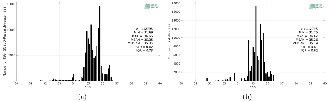
Figure 2: Histograms of SSS from TSG (GOSUD-Research-vessel) (a) and Aquarius SSS L3 OR v5 - Monthly (NASA-GSFC) (b) considering all match-up pairs per bins of 0.1 over the South Pacific Ocean Pi-MEP region and for the full satellite product period.
