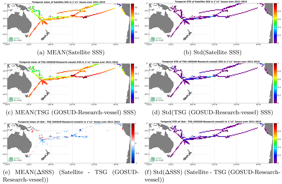
Figure 6: Temporal mean (left) and Std (right) of SSS from Aquarius SSS L3 OR v5 - Monthly (NASA-GSFC) (top), TSG (GOSUD-Research-vessel) (middle), and of \Delta SSS (Satellite - TSG (GOSUD-Research-vessel)). Only match-up pairs are used to generate these maps.
