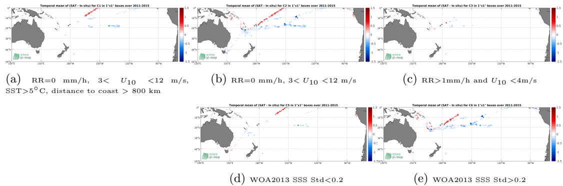
Figure 12: Temporal mean gridded over spatial boxes of size 1^\circ \times 1^\circ of \Delta SSS (Aquarius-L3-OR-V5-MONTHLY-1DEG - TSG-GOSUD-Research-vessel) for 5 different subdatasets corresponding to:RR=0 mm/h, 3 < U_{10} < 12 m/s, SST >5^\circ C, distance to coast > 800 km (a), RR=0 mm/h, 3 < U_{10} < 12 m/s (b), RR >1 mm/h and U_{10} < 4 m/s (c), WOA2013 SSS Std <0.2 (d), WOA2013 SSS Std >0.2 (e).
