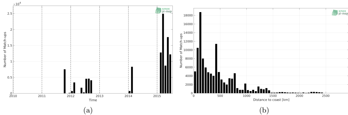
Figure 1: Number of match-ups between TSG-GOSUD-Research-vessel and Aquarius-L3-OR-V5-MONTHLY-1DEG SSS as a function of time (a) and as function of the distance to coast (b) over the South Pacific Ocean Pi-MEP region and for the full satellite product period.
