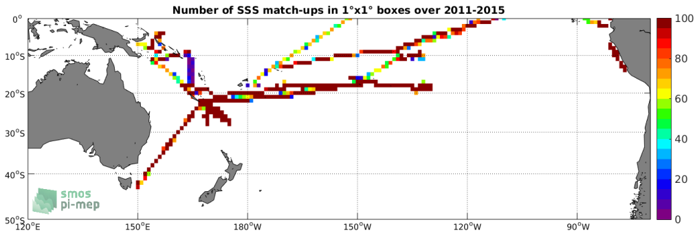
Figure 4: Number of SSS match-ups between TSG-GOSUD-Research-vessel SSS and the Aquarius-L3-OR-V5-MONTHLY-1DEG SSS product for the South Pacific Ocean Pi-MEP region over 1^\circ \times 1^\circ boxes and for the full satellite product period.
