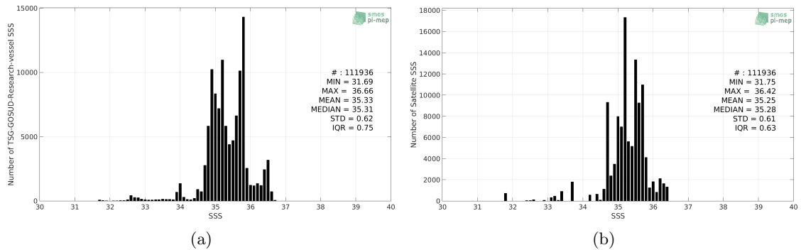
Figure 2: Histograms of SSS from TSG-GOSUD-Research-vessel (a) and Aquarius-L3-OR-V5-MONTHLY-1DEG (b) considering all match-up pairs per bins of 0.1 over the South Pacific Ocean Pi-MEP region and for the full satellite product period.
