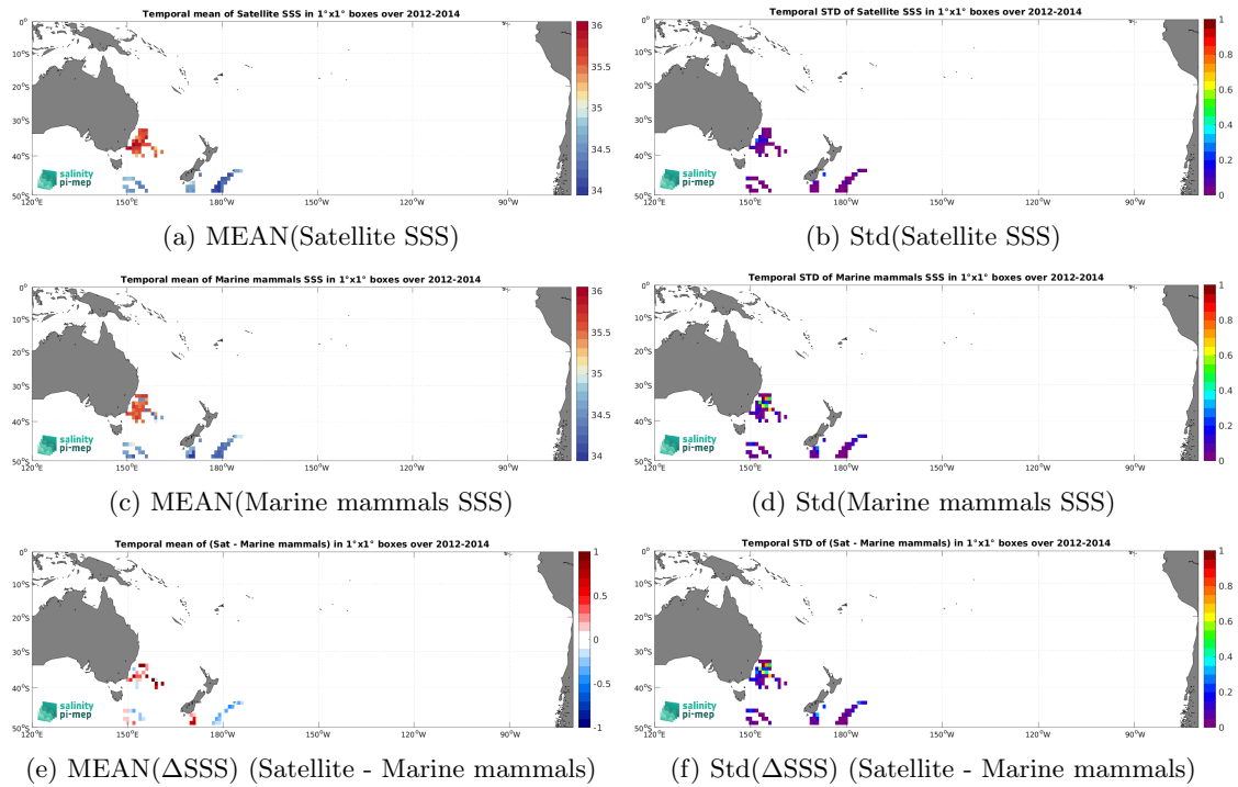
Figure 7: Temporal mean (left) and Std (right) of SSS from Aquarius SSS L3 OR v5 - Monthly (NASA-GSFC) (top), Marine mammals (middle), and of \Delta SSS (Satellite - Marine mammals). Only match-up pairs are used to generate these maps.
