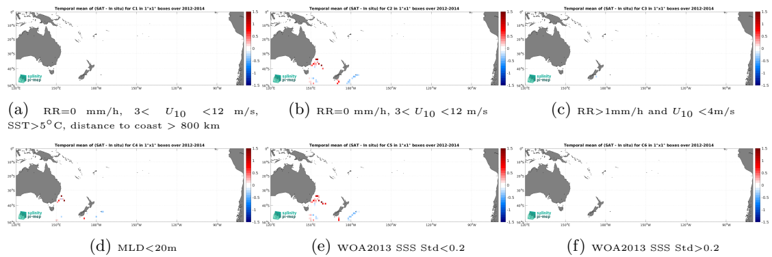
Figure 14: Temporal mean gridded over spatial boxes of size 1^\circ \times 1^\circ of \Delta SSS (Aquarius SSS L3 OR v5 - Monthly (NASA-GSFC) - Marine mammals) for 6 different subdatasets corresponding to:RR=0 mm/h, 3 < U_{10} < 12 m/s, SST>5°C, distance to coast > 800 km (a), RR=0 mm/h, 3 < U_{10} < 12 m/s (b), RR>1mm/h and U_{10} < 4 m/s (c),MLD<20m (d),WOA2013 SSS Std<0.2 (e),WOA2013 SSS Std>0.2 (f).
