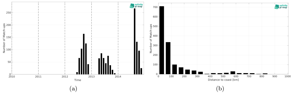
Figure 2: Number of match-ups between Marine mammals and Aquarius SSS L3 OR v5 - Monthly (NASA-GSFC) SSS as a function of time (a) and as function of the distance to coast (b) over the South Pacific Ocean Pi-MEP region and for the full satellite product period.
