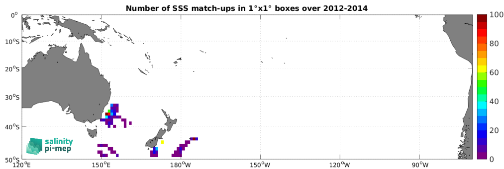
Figure 5: Number of SSS match-ups between Marine mammals SSS and the Aquarius SSS L3 OR v5 - Monthly (NASA-GSFC) SSS product for the South Pacific Ocean Pi-MEP region over 1^\circ \times 1^\circ boxes and for the full satellite product period.
