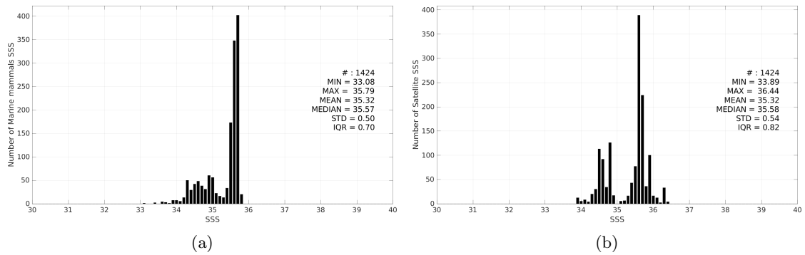
Figure 3: Histograms of SSS from Marine mammals (a) and Aquarius SSS L3 OR v5 - Monthly (NASA-GSFC) (b) considering all match-up pairs per bins of 0.1 over the South Pacific Ocean Pi-MEP region and for the full satellite product period.
