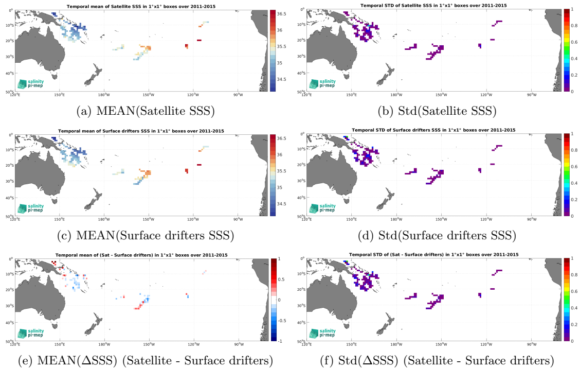
Figure 6: Temporal mean (left) and Std (right) of SSS from Aquarius SSS L3 OR v5 - Monthly (NASA-GSFC) (top), Surface drifters (middle), and of \Delta SSS (Satellite - Surface drifters). Only match-up pairs are used to generate these maps.
