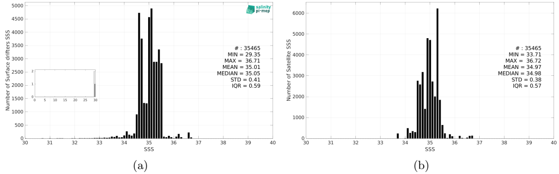
Figure 3: Histograms of SSS from Surface drifters (a) and Aquarius SSS L3 OR v5 - Monthly (NASA-GSFC) (b) considering all match-up pairs per bins of 0.1 over the South Pacific Ocean Pi-MEP region and for the full satellite product period.
