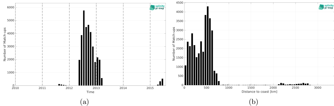
Figure 2: Number of match-ups between Surface drifters and Aquarius SSS L3 OR v5 - Monthly (NASA-GSFC) SSS as a function of time (a) and as function of the distance to coast (b) over the South Pacific Ocean Pi-MEP region and for the full satellite product period.
