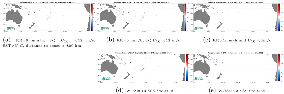
Figure 13: Temporal mean gridded over spatial boxes of size 1^\circ \times 1^\circ of \Delta SSS (Aquarius SSS L3 OR v5 - Monthly (NASA-GSFC) - Surface drifters) for 5 different subdatasets corresponding to:RR=0 mm/h, 3 < U_{10} < 12 m/s, SST >5^\circ\text{C} , distance to coast > 800 km (a), RR=0 mm/h, 3 < U_{10} < 12 m/s (b), RR >1 mm/h and U_{10} < 4 m/s (c), WOA2013 SSS Std <0.2 (d), WOA2013 SSS Std >0.2 (e).
