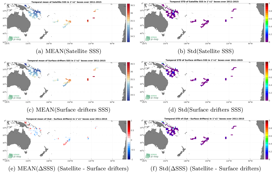
Figure 5: Temporal mean (left) and Std (right) of SSS from Aquarius SSS L3 OR v5 - Monthly (NASA-GSFC) (top), Surface drifters (middle), and of \Delta SSS (Satellite - Surface drifters). Only match-up pairs are used to generate these maps.
