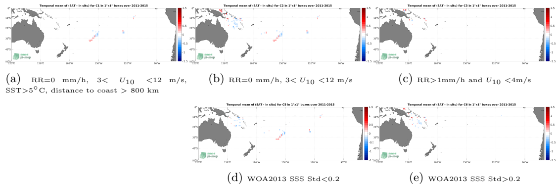
Figure 11: Temporal mean gridded over spatial boxes of size 1^\circ \times 1^\circ of \Delta SSS (Aquarius SSS L3 OR v5 - Monthly (NASA-GSFC) - Surface drifters) for 5 different subdatasets corresponding to:RR=0 mm/h, 3 < U_{10} < 12 m/s, SST >5^\circ\text{C} , distance to coast > 800 km (a), RR=0 mm/h, 3 < U_{10} < 12 m/s (b), RR >1 mm/h and U_{10} < 4 m/s (c), WOA2013 SSS Std <0.2 (d), WOA2013 SSS Std >0.2 (e).
