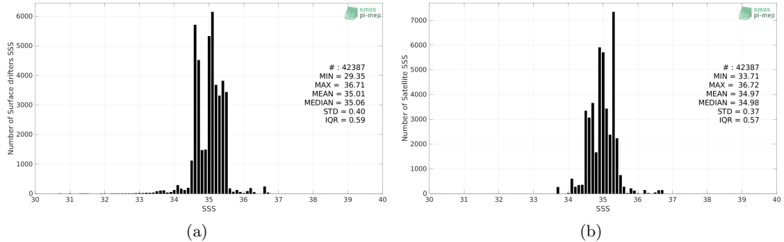
Figure 2: Histograms of SSS from Surface drifters (a) and Aquarius SSS L3 OR v5 - Monthly (NASA-GSFC) (b) considering all match-up pairs per bins of 0.1 over the South Pacific Ocean Pi-MEP region and for the full satellite product period.
