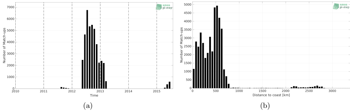
Figure 1: Number of match-ups between Surface drifters and Aquarius SSS L3 OR v5 - Monthly (NASA-GSFC) SSS as a function of time (a) and as function of the distance to coast (b) over the South Pacific Ocean Pi-MEP region and for the full satellite product period.
