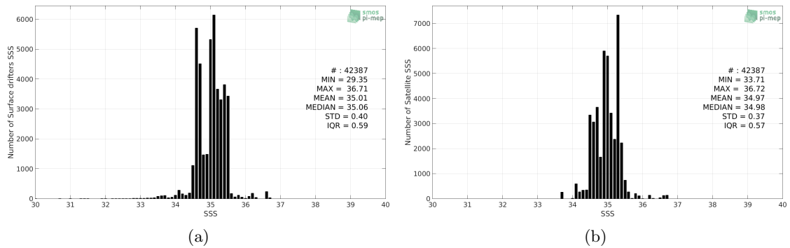
Figure 2: Histograms of SSS from Surface drifters (a) and Aquarius-L3-OR-V5-MONTHLY-1DEG (b) considering all match-up pairs per bins of 0.1 over the South Pacific Ocean Pi-MEP region and for the full satellite product period.
