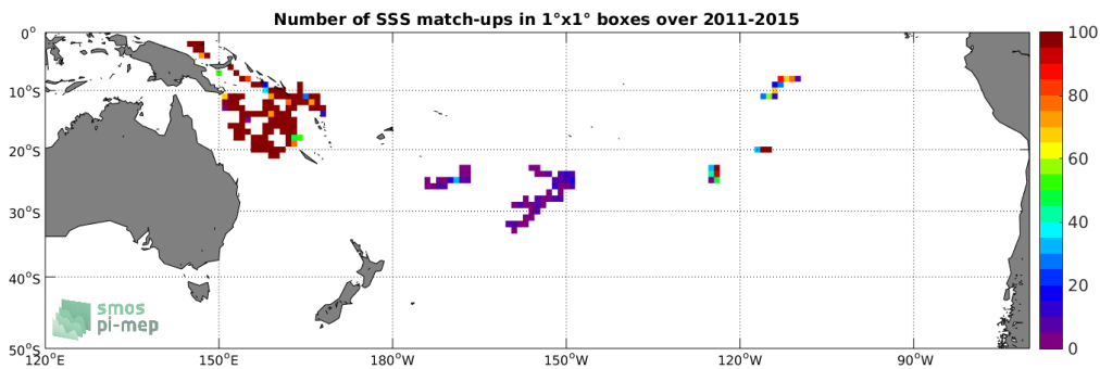
Figure 3: Number of SSS match-ups between Surface drifters SSS and the Aquarius-L3-OR-V5-MONTHLY-1DEG SSS product for the South Pacific Ocean Pi-MEP region over 1°x1° boxes and for the full satellite product period.
