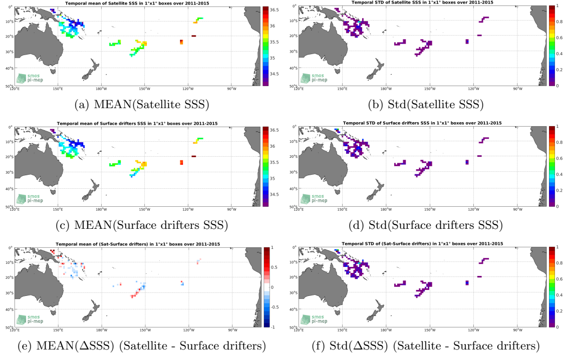
Figure 5: Temporal mean (left) and Std (right) of SSS from Aquarius-L3-OR-V5-MONTHLY-1DEG (top), Surface drifters (middle), and of \Delta SSS (Satellite - Surface drifters). Only match-up pairs are used to generate these maps.
