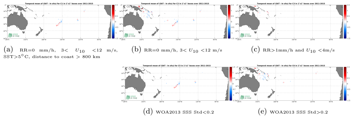
Figure 11: Temporal mean gridded over spatial boxes of size 1^\circ \times 1^\circ of \Delta SSS (Aquarius-L3-OR-V5-MONTHLY-1DEG - Surface drifters) for 5 different subdatasets corresponding to:RR=0 mm/h, 3 < U_{10} < 12 m/s, SST >5^\circ C, distance to coast > 800 km (a), RR=0 mm/h, 3 < U_{10} < 12 m/s (b), RR >1 mm/h and U_{10} < 4 m/s (c), WOA2013 SSS Std <0.2 (d), WOA2013 SSS Std >0.2 (e).
