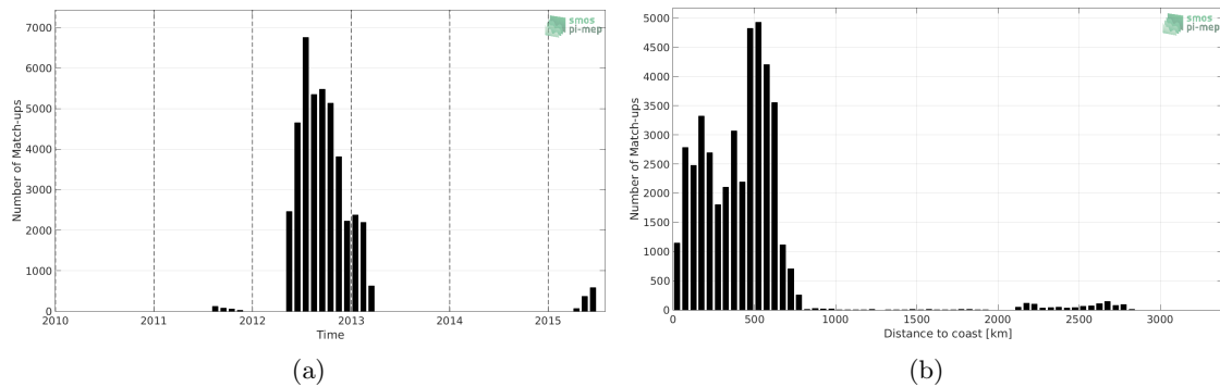
Figure 1: Number of match-ups between Surface drifters and Aquarius-L3-OR-V5-MONTHLY-1DEG SSS as a function of time (a) and as function of the distance to coast (b) over the South Pacific Ocean Pi-MEP region and for the full satellite product period.
