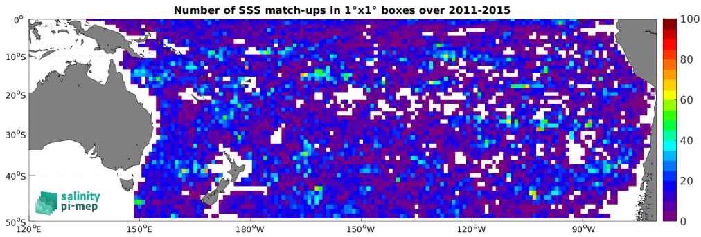
Figure 5: Number of SSS match-ups between Argo SSS and the Aquarius SSS L3 OR v5 - Monthly (NASA-GSFC) SSS product for the South Pacific Ocean Pi-MEP region over 1^\circ \times 1^\circ boxes and for the full satellite product period.
