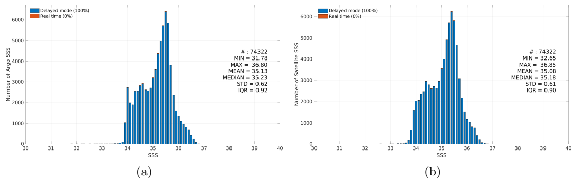
Figure 3: Histograms of SSS from Argo (a) and Aquarius SSS L3 OR v5 - Monthly (NASA-GSFC) (b) considering all match-up pairs per bins of 0.1 over the South Pacific Ocean Pi-MEP region and for the full satellite product period.
