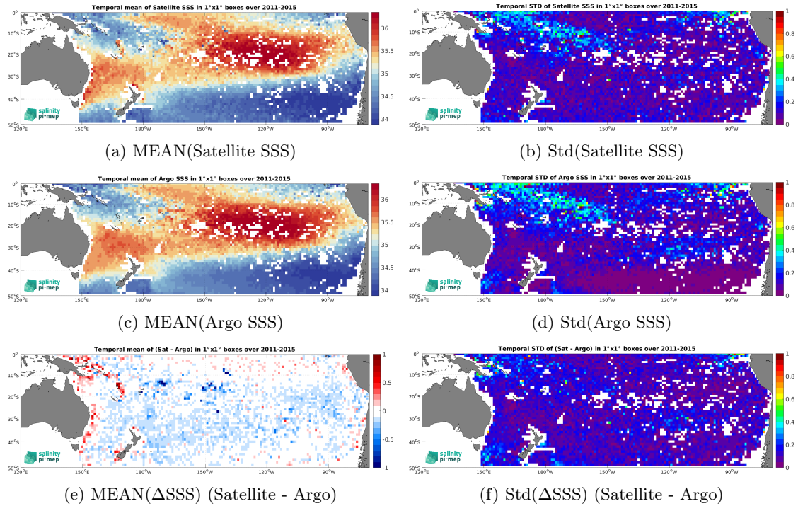
Figure 7: Temporal mean (left) and Std (right) of SSS from Aquarius SSS L3 OR v5 - Monthly (NASA-GSFC) (top), Argo (middle), and of \Delta SSS (Satellite - Argo). Only match-up pairs are used to generate these maps.
