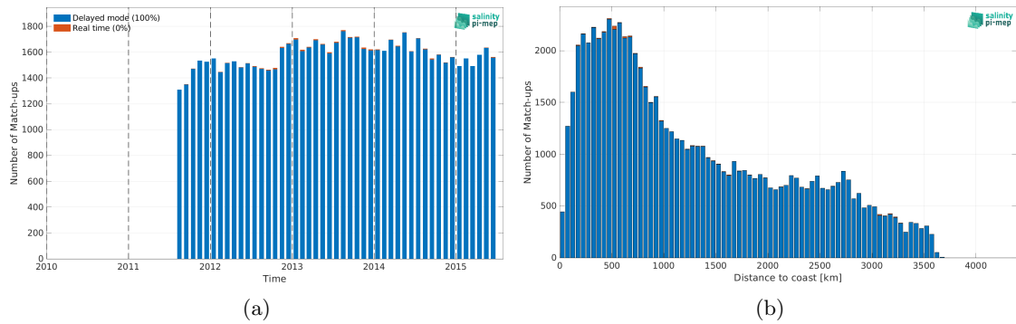
Figure 2: Number of match-ups between Argo and Aquarius SSS L3 OR v5 - Monthly (NASA-GSFC) SSS as a function of time (a) and as function of the distance to coast (b) over the South Pacific Ocean Pi-MEP region and for the full satellite product period.
