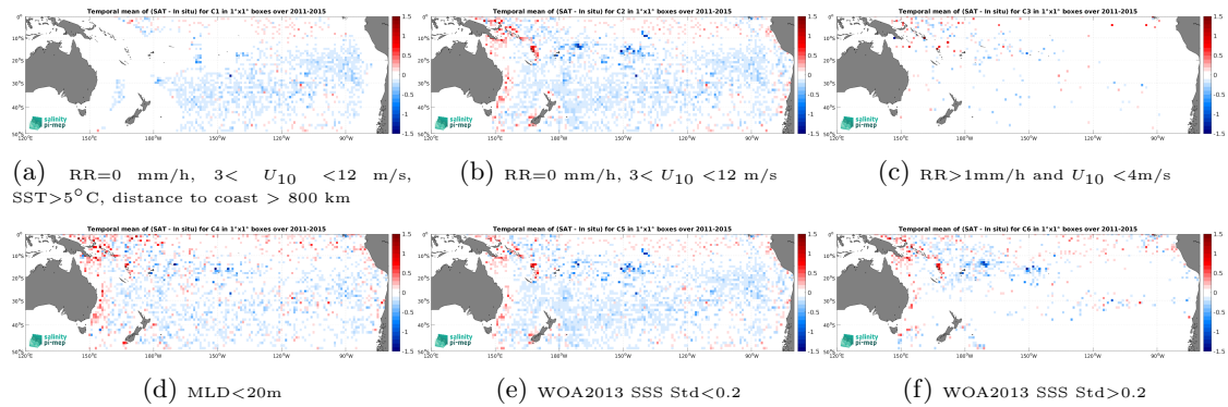
Figure 14: Temporal mean gridded over spatial boxes of size 1^\circ \times 1^\circ of \Delta SSS (Aquarius SSS L3 OR v5 - Monthly (NASA-GSFC) - Argo) for 6 different subdatasets corresponding to:RR=0 mm/h, 3 < U_{10} < 12 m/s, SST >5^\circ C, distance to coast > 800 km (a), RR=0 mm/h, 3 < U_{10} < 12 m/s (b), RR >1 mm/h and U_{10} < 4 m/s (c),MLD <20 m (d),WOA2013 SSS Std <0.2 (e),WOA2013 SSS Std >0.2 (f).
