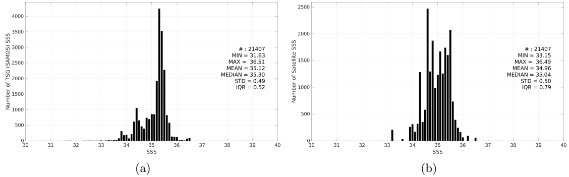
Figure 3: Histograms of SSS from TSG (SAMOS) (a) and Aquarius SSS L3 OR v5 - Monthly - Rain mask (NASA-GSFC) (b) considering all match-up pairs per bins of 0.1 over the South Pacific Ocean Pi-MEP region and for the full satellite product period.
