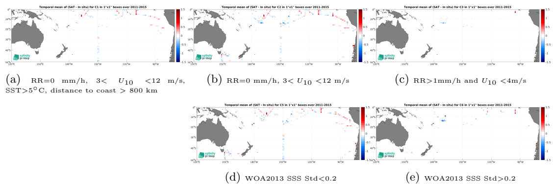
Figure 14: Temporal mean gridded over spatial boxes of size 1^\circ \times 1^\circ of \Delta\text{SSS} (Aquarius SSS L3 OR v5 - Monthly - Rain mask (NASA-GSFC) - TSG (SAMOS)) for 5 different subdatasets corresponding to:RR=0 mm/h, 3 < U_{10} < 12 m/s, SST >5^\circ\text{C} , distance to coast > 800 km (a), RR=0 mm/h, 3 < U_{10} < 12 m/s (b), RR >1 mm/h and U_{10} < 4 m/s (c), WOA2013 SSS Std <0.2 (d), WOA2013 SSS Std >0.2 (e).
