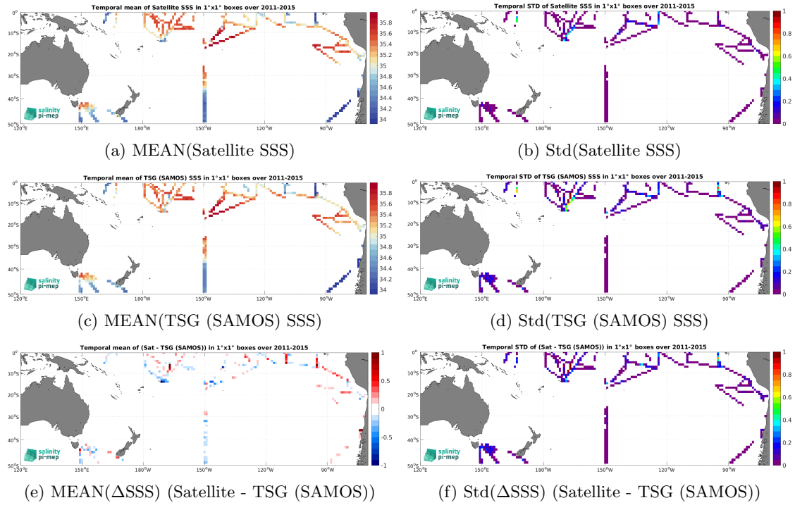
Figure 7: Temporal mean (left) and Std (right) of SSS from Aquarius SSS L3 OR v5 - Monthly - Rain mask (NASA-GSFC) (top), TSG (SAMOS) (middle), and of \Delta SSS (Satellite - TSG (SAMOS)). Only match-up pairs are used to generate these maps.
