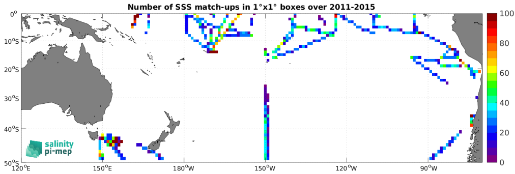
Figure 5: Number of SSS match-ups between TSG (SAMOS) SSS and the Aquarius SSS L3 OR v5 - Monthly - Rain mask (NASA-GSFC) SSS product for the South Pacific Ocean Pi-MEP region over 1^\circ \times 1^\circ boxes and for the full satellite product period.
