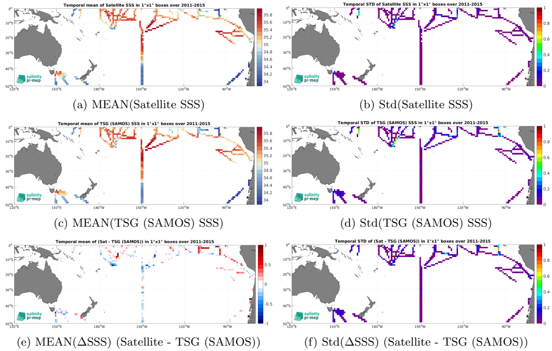
Figure 6: Temporal mean (left) and Std (right) of SSS from Aquarius SSS L3 OR v5 - Monthly - Rain mask (NASA-GSFC) (top), TSG (SAMOS) (middle), and of \Delta SSS (Satellite - TSG (SAMOS)). Only match-up pairs are used to generate these maps.
