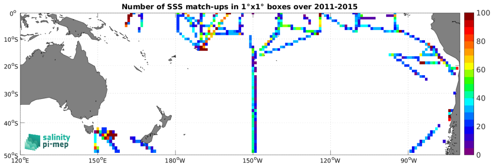
Figure 4: Number of SSS match-ups between TSG (SAMOS) SSS and the Aquarius SSS L3 OR v5 - Monthly - Rain mask (NASA-GSFC) SSS product for the South Pacific Ocean Pi-MEP region over 1^\circ \times 1^\circ boxes and for the full satellite product period.
