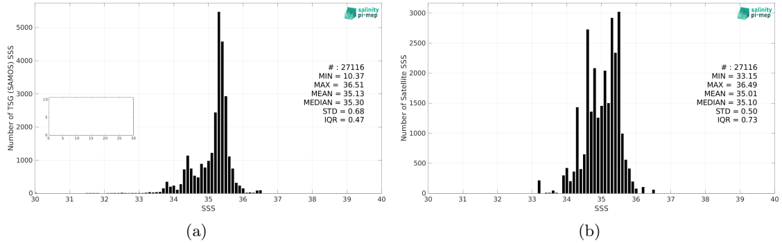
Figure 2: Histograms of SSS from TSG (SAMOS) (a) and Aquarius SSS L3 OR v5 - Monthly - Rain mask (NASA-GSFC) (b) considering all match-up pairs per bins of 0.1 over the South Pacific Ocean Pi-MEP region and for the full satellite product period.
