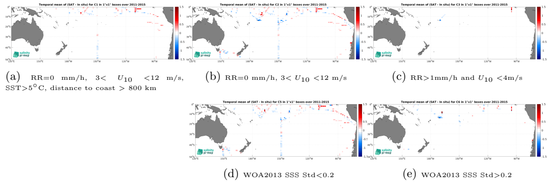
Figure 12: Temporal mean gridded over spatial boxes of size 1^\circ \times 1^\circ of \Delta SSS (Aquarius SSS L3 OR v5 - Monthly - Rain mask (NASA-GSFC) - TSG (SAMOS)) for 5 different subdatasets corresponding to:RR=0 mm/h, 3 < U_{10} < 12 m/s, SST >5^\circ\text{C} , distance to coast > 800 km (a), RR=0 mm/h, 3 < U_{10} < 12 m/s (b), RR >1 mm/h and U_{10} < 4 m/s (c), WOA2013 SSS Std <0.2 (d), WOA2013 SSS Std >0.2 (e).
