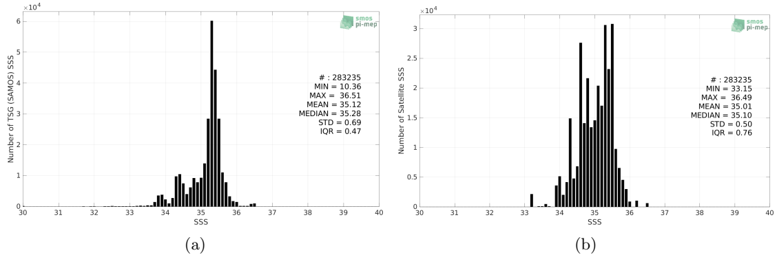
Figure 2: Histograms of SSS from TSG (SAMOS) (a) and Aquarius SSS L3 OR v5 - Monthly - Rain mask (NASA-GSFC) (b) considering all match-up pairs per bins of 0.1 over the South Pacific Ocean Pi-MEP region and for the full satellite product period.
