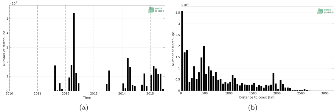
Figure 1: Number of match-ups between TSG (SAMOS) and Aquarius SSS L3 OR v5 - Monthly - Rain mask (NASA-GSFC) SSS as a function of time (a) and as function of the distance to coast (b) over the South Pacific Ocean Pi-MEP region and for the full satellite product period.
