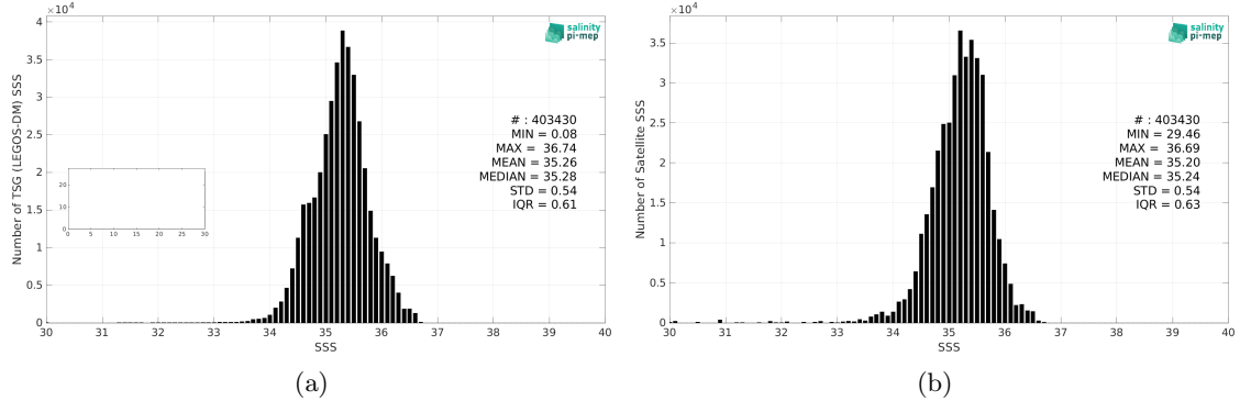
Figure 2: Histograms of SSS from TSG (LEGOS-DM) (a) and Aquarius SSS L3 OR v5 - Monthly - Rain mask (NASA-GSFC) (b) considering all match-up pairs per bins of 0.1 over the South Pacific Ocean Pi-MEP region and for the full satellite product period.
