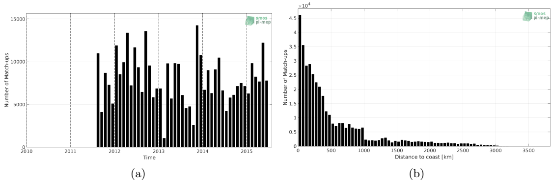
Figure 1: Number of match-ups between TSG-LEGOS-DM and Aquarius-L3-OR-V5-MONTHLY-RAIN-MASK-1DEG SSS as a function of time (a) and as function of the distance to coast (b) over the South Pacific Ocean Pi-MEP region and for the full satellite product period.
