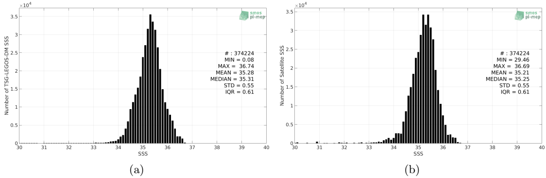
Figure 2: Histograms of SSS from TSG-LEGOS-DM (a) and Aquarius-L3-OR-V5-MONTHLY-RAIN-MASK-1DEG (b) considering all match-up pairs per bins of 0.1 over the South Pacific Ocean Pi-MEP region and for the full satellite product period.
