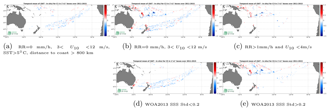
Figure 12: Temporal mean gridded over spatial boxes of size 1^\circ \times 1^\circ of \Delta SSS (Aquarius-L3-OR-V5-MONTHLY-RAIN-MASK-1DEG - TSG-LEGOS-DM) for 5 different subdatasets corresponding to: RR=0 mm/h, 3 < U_{10} < 12 m/s, SST > 5^\circ C, distance to coast > 800 km (a), RR=0 mm/h, 3 < U_{10} < 12 m/s (b), RR > 1 mm/h and U_{10} < 4 m/s (c), WOA2013 SSS Std < 0.2 (d), WOA2013 SSS Std > 0.2 (e).
