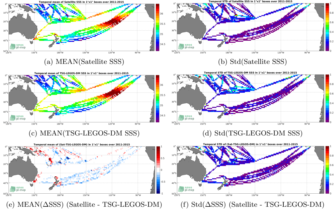
Figure 6: Temporal mean (left) and Std (right) of SSS from Aquarius-L3-OR-V5-MONTHLY-RAIN-MASK-1DEG (top), TSG-LEGOS-DM (middle), and of \Delta SSS (Satellite - TSG-LEGOS-DM). Only match-up pairs are used to generate these maps.
