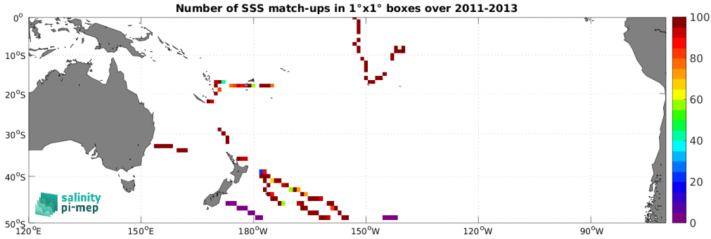
Figure 5: Number of SSS match-ups between TSG (GOSUD-Sailing-ship) SSS and the Aquarius SSS L3 OR v5 - Monthly - Rain mask (NASA-GSFC) SSS product for the South Pacific Ocean Pi-MEP region over 1^\circ \times 1^\circ boxes and for the full satellite product period.
