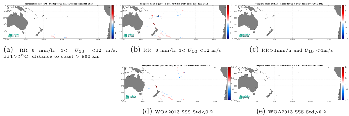
Figure 14: Temporal mean gridded over spatial boxes of size 1^\circ \times 1^\circ of \Delta SSS (Aquarius SSS L3 OR v5 - Monthly - Rain mask (NASA-GSFC) - TSG (GOSUD-Sailing-ship)) for 5 different subdatasets corresponding to:RR=0 mm/h, 3 < U_{10} < 12 m/s, SST >5^\circ\text{C} , distance to coast > 800 km (a), RR=0 mm/h, 3 < U_{10} < 12 m/s (b), RR >1 mm/h and U_{10} < 4 m/s (c), WOA2013 SSS Std <0.2 (d), WOA2013 SSS Std >0.2 (e).
