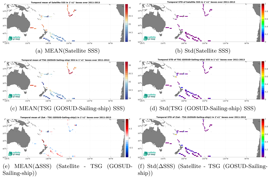
Figure 7: Temporal mean (left) and Std (right) of SSS from Aquarius SSS L3 OR v5 - Monthly - Rain mask (NASA-GSFC) (top), TSG (GOSUD-Sailing-ship) (middle), and of \Delta SSS (Satellite - TSG (GOSUD-Sailing-ship)). Only match-up pairs are used to generate these maps.
