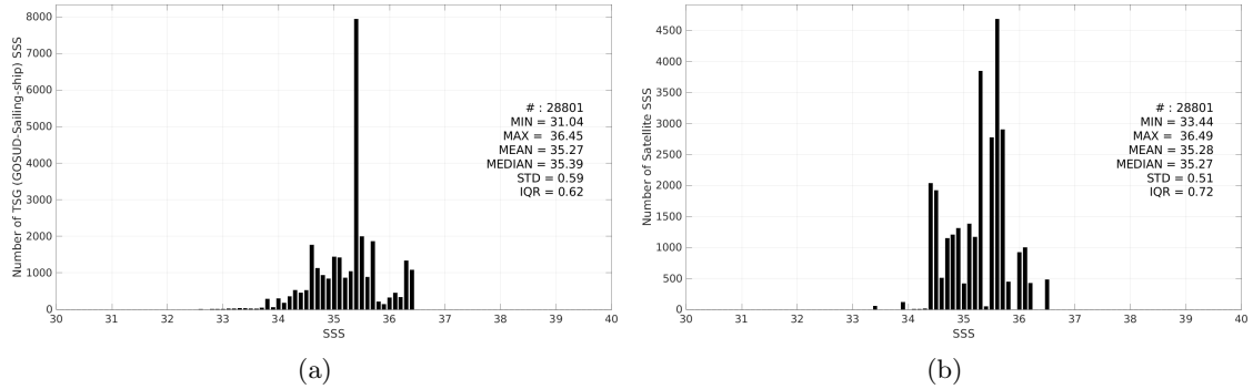
Figure 3: Histograms of SSS from TSG (GOSUD-Sailing-ship) (a) and Aquarius SSS L3 OR v5 - Monthly - Rain mask (NASA-GSFC) (b) considering all match-up pairs per bins of 0.1 over the South Pacific Ocean Pi-MEP region and for the full satellite product period.
