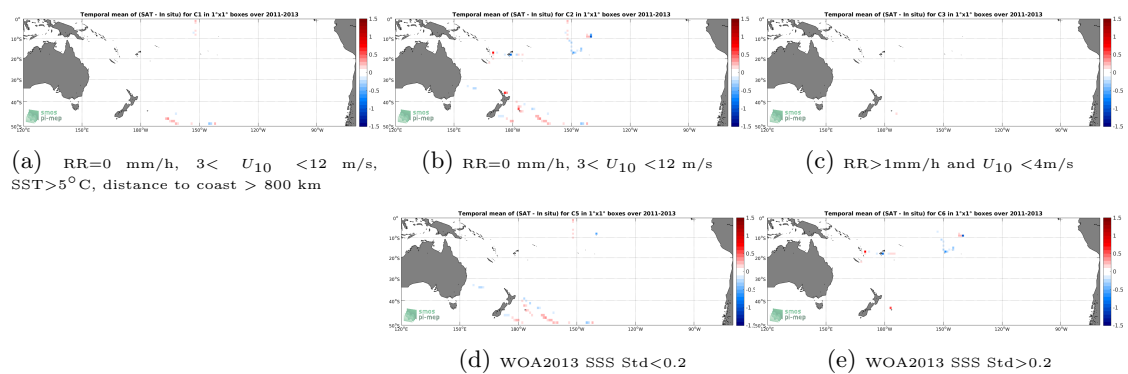
Figure 12: Temporal mean gridded over spatial boxes of size 1^\circ \times 1^\circ of \Delta\text{SSS} (Aquarius SSS L3 OR v5 - Monthly - Rain mask (NASA-GSFC) - TSG (GOSUD-Sailing-ship)) for 5 different subdatasets corresponding to:RR=0 mm/h, 3 < U_{10} < 12 m/s, SST>5°C, distance to coast > 800 km (a), RR=0 mm/h, 3 < U_{10} < 12 m/s (b), RR>1mm/h and U_{10} < 4 m/s (c), WOA2013 SSS Std<0.2 (d), WOA2013 SSS Std>0.2 (e).
