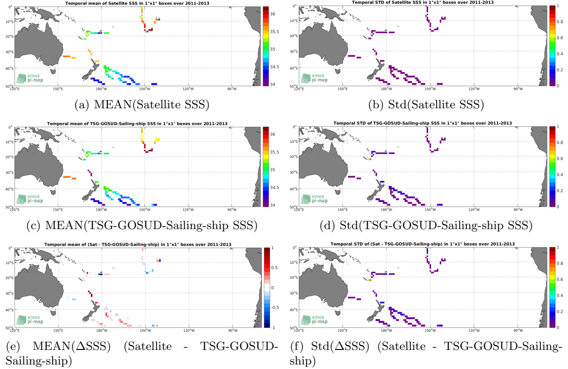
Figure 6: Temporal mean (left) and Std (right) of SSS from Aquarius-L3-OR-V5-MONTHLY-RAIN-MASK-1DEG (top), TSG-GOSUD-Sailing-ship (middle), and of \Delta SSS (Satellite - TSG-GOSUD-Sailing-ship). Only match-up pairs are used to generate these maps.
