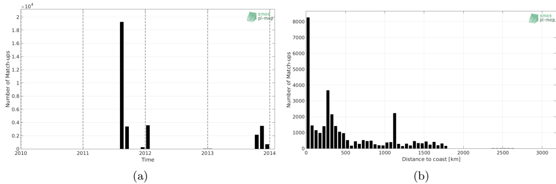
Figure 1: Number of match-ups between TSG-GOSUD-Sailing-ship and Aquarius-L3-OR-V5-MONTHLY-RAIN-MASK-1DEG SSS as a function of time (a) and as function of the distance to coast (b) over the South Pacific Ocean Pi-MEP region and for the full satellite product period.
