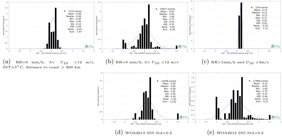
Figure 13: Normalized histogram of \Delta SSS (Aquarius-L3-OR-V5-MONTHLY-RAIN-MASK-1DEG - TSG-GOSUD-Sailing-ship) for 5 different subdatasets corresponding to: RR=0 mm/h, 3 < U_{10} < 12 m/s, SST>5°C, distance to coast > 800 km (a), RR=0 mm/h, 3 < U_{10} < 12 m/s (b), RR>1mm/h and U_{10} < 4 m/s (c), WOA2013 SSS Std<0.2 (d), WOA2013 SSS Std>0.2 (e).
