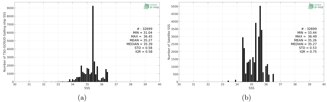
Figure 2: Histograms of SSS from TSG-GOSUD-Sailing-ship (a) and Aquarius-L3-OR-V5-MONTHLY-RAIN-MASK-1DEG (b) considering all match-up pairs per bins of 0.1 over the South Pacific Ocean Pi-MEP region and for the full satellite product period.
