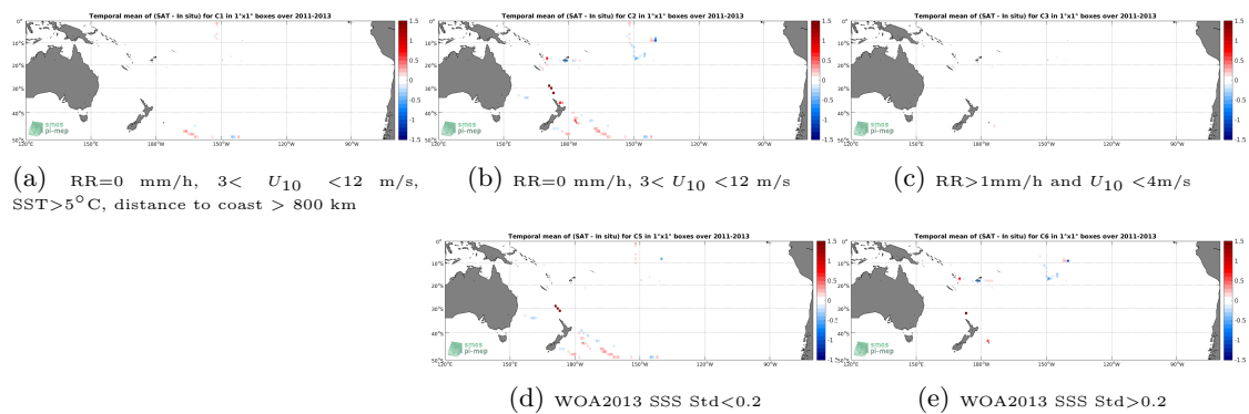
Figure 12: Temporal mean gridded over spatial boxes of size 1^\circ \times 1^\circ of \Delta SSS (Aquarius-L3-OR-V5-MONTHLY-RAIN-MASK-1DEG - TSG-GOSUD-Sailing-ship) for 5 different subdatasets corresponding to:RR=0 mm/h, 3 < U_{10} < 12 m/s, SST >5^\circ C, distance to coast > 800 km (a), RR=0 mm/h, 3 < U_{10} < 12 m/s (b), RR >1 mm/h and U_{10} < 4 m/s (c), WOA2013 SSS Std <0.2 (d), WOA2013 SSS Std >0.2 (e).
