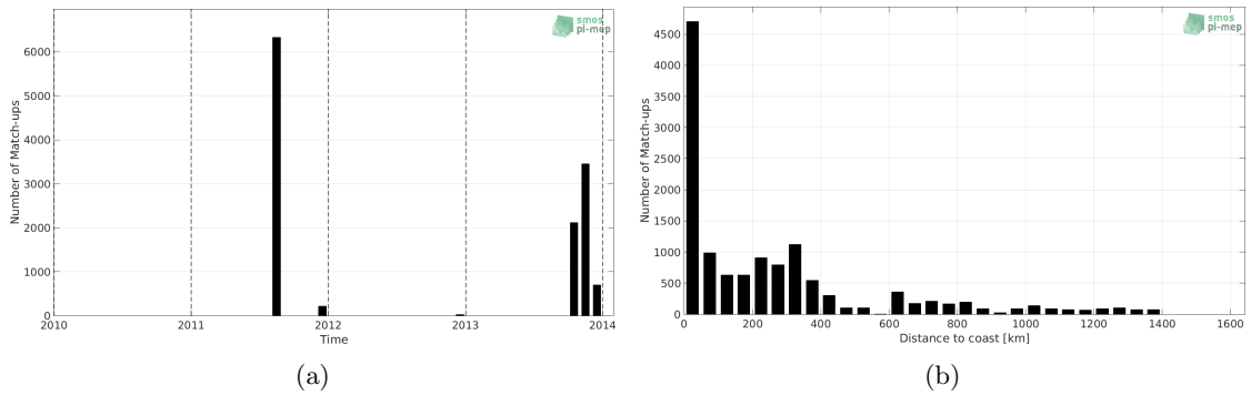
Figure 1: Number of match-ups between TSG-GOSUD-Sailing-ship and Aquarius-L3-OR-V5-MONTHLY-RAIN-MASK-1DEG SSS as a function of time (a) and as function of the distance to coast (b) over the South Pacific Ocean Pi-MEP region and for the full satellite product period.
