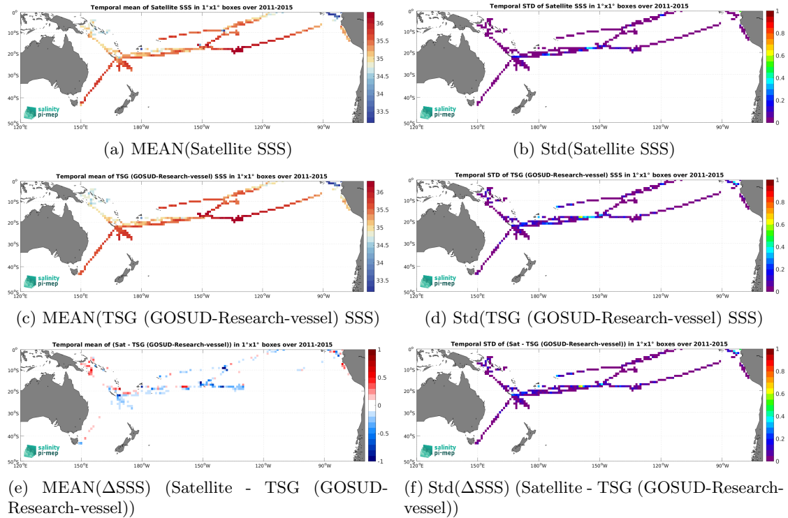
Figure 7: Temporal mean (left) and Std (right) of SSS from Aquarius SSS L3 OR v5 - Monthly - Rain mask (NASA-GSFC) (top), TSG (GOSUD-Research-vessel) (middle), and of \Delta SSS (Satellite - TSG (GOSUD-Research-vessel)). Only match-up pairs are used to generate these maps.
