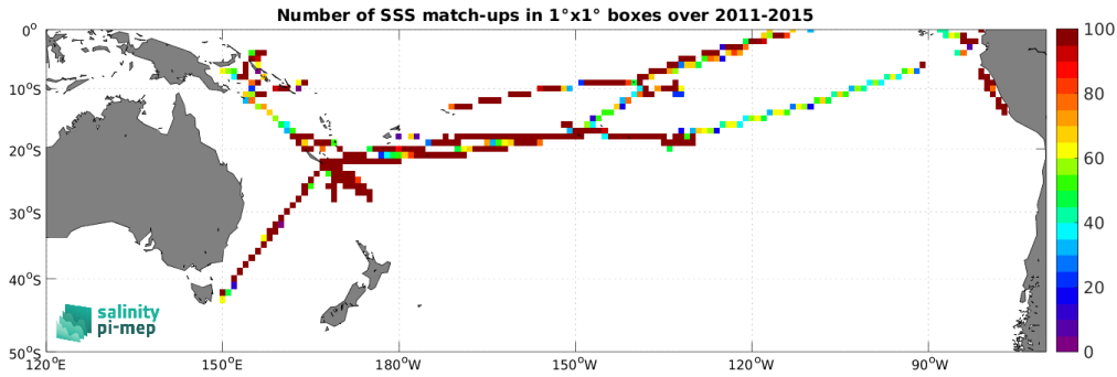
Figure 5: Number of SSS match-ups between TSG (GOSUD-Research-vessel) SSS and the Aquarius SSS L3 OR v5 - Monthly - Rain mask (NASA-GSFC) SSS product for the South Pacific Ocean Pi-MEP region over 1^\circ \times 1^\circ boxes and for the full satellite product period.
