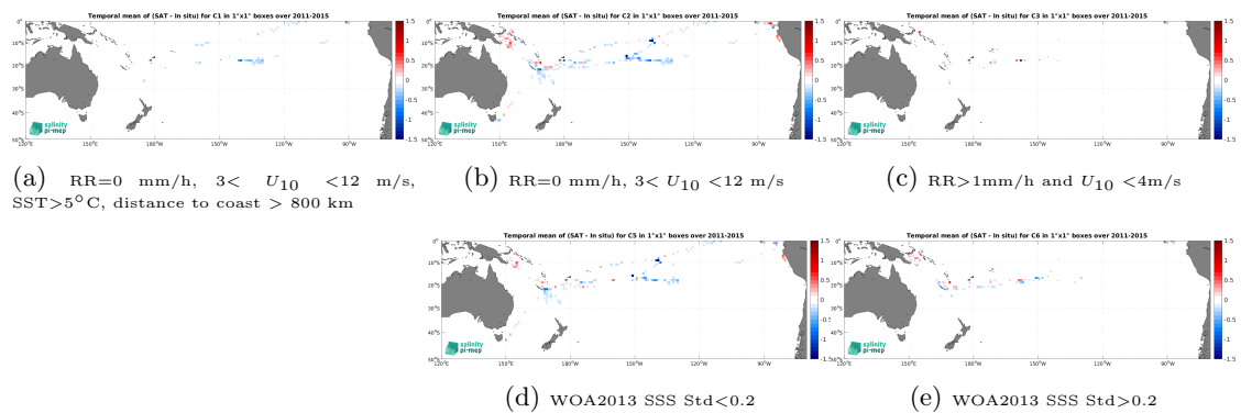
Figure 14: Temporal mean gridded over spatial boxes of size 1^\circ \times 1^\circ of \Delta SSS (Aquarius SSS L3 OR v5 - Monthly - Rain mask (NASA-GSFC) - TSG (GOSUD-Research-vessel)) for 5 different subdatasets corresponding to:RR=0 mm/h, 3 < U_{10} < 12 m/s, SST >5^\circ\text{C} , distance to coast > 800 km (a), RR=0 mm/h, 3 < U_{10} < 12 m/s (b), RR >1 mm/h and U_{10} < 4 m/s (c), WOA2013 SSS Std <0.2 (d), WOA2013 SSS Std >0.2 (e).
