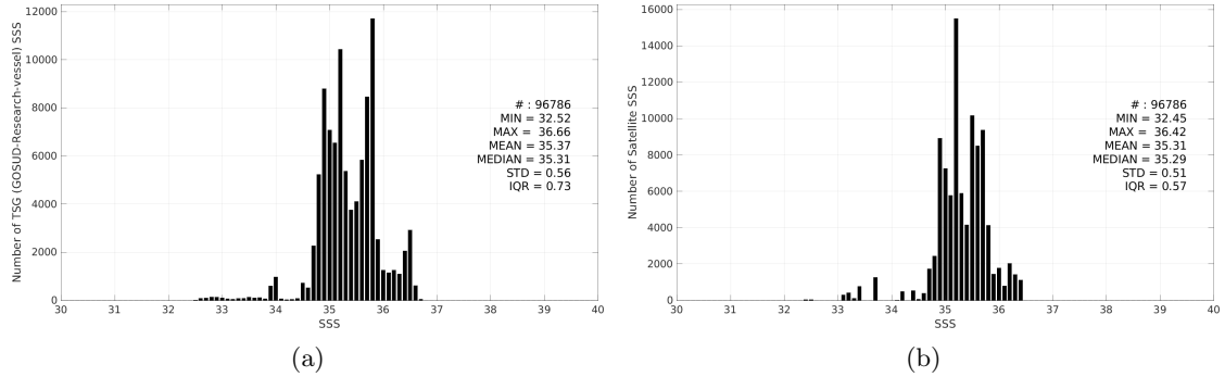
Figure 3: Histograms of SSS from TSG (GOSUD-Research-vessel) (a) and Aquarius SSS L3 OR v5 - Monthly - Rain mask (NASA-GSFC) (b) considering all match-up pairs per bins of 0.1 over the South Pacific Ocean Pi-MEP region and for the full satellite product period.
