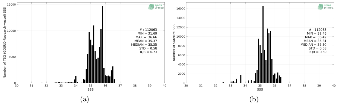
Figure 2: Histograms of SSS from TSG (GOSUD-Research-vessel) (a) and Aquarius SSS L3 OR v5 - Monthly - Rain mask (NASA-GSFC) (b) considering all match-up pairs per bins of 0.1 over the South Pacific Ocean Pi-MEP region and for the full satellite product period.
