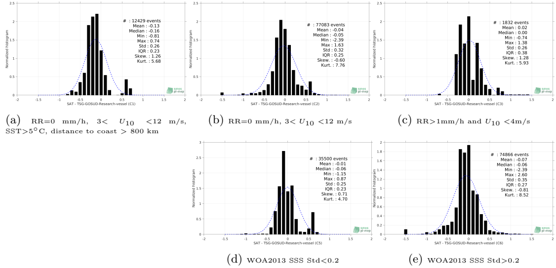
Figure 13: Normalized histogram of \Delta\text{SSS} (Aquarius-L3-OR-V5-MONTHLY-RAIN-MASK-1DEG - TSG-GOSUD-Research-vessel) for 5 different subdatasets corresponding to: RR=0 mm/h, 3 < U_{10} < 12 m/s, SST > 5^\circ\text{C} , distance to coast > 800 km (a), RR=0 mm/h, 3 < U_{10} < 12 m/s (b), RR > 1 mm/h and U_{10} < 4 m/s (c), WOA2013 SSS Std < 0.2 (d), WOA2013 SSS Std > 0.2 (e).
