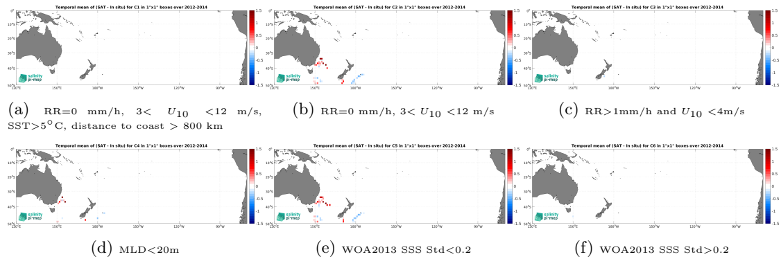
Figure 14: Temporal mean gridded over spatial boxes of size 1^\circ \times 1^\circ of \Delta SSS (Aquarius SSS L3 OR v5 - Monthly - Rain mask (NASA-GSFC) - Marine mammals) for 6 different subdatasets corresponding to:RR=0 mm/h, 3 < U_{10} < 12 m/s, SST >5^\circ C, distance to coast > 800 km (a), RR=0 mm/h, 3 < U_{10} < 12 m/s (b), RR >1 mm/h and U_{10} < 4 m/s (c),MLD <20 m (d),WOA2013 SSS Std <0.2 (e),WOA2013 SSS Std >0.2 (f).
