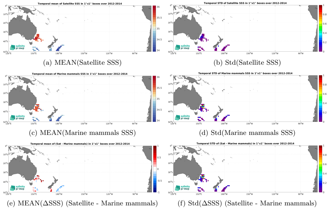
Figure 7: Temporal mean (left) and Std (right) of SSS from Aquarius SSS L3 OR v5 - Monthly - Rain mask (NASA-GSFC) (top), Marine mammals (middle), and of \Delta SSS (Satellite - Marine mammals). Only match-up pairs are used to generate these maps.
