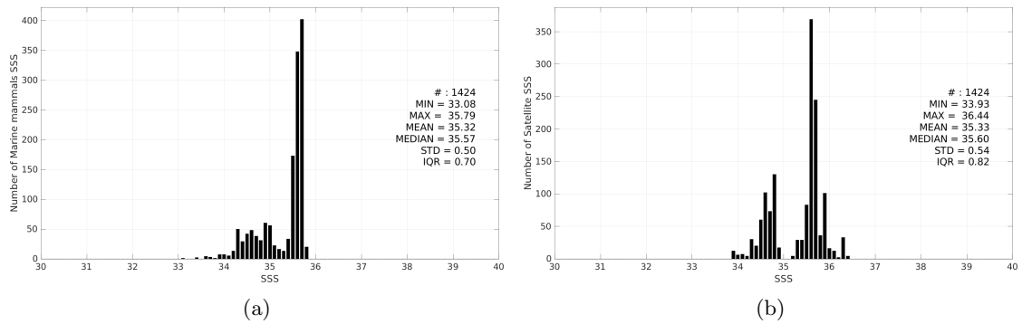
Figure 3: Histograms of SSS from Marine mammals (a) and Aquarius SSS L3 OR v5 - Monthly - Rain mask (NASA-GSFC) (b) considering all match-up pairs per bins of 0.1 over the South Pacific Ocean Pi-MEP region and for the full satellite product period.
