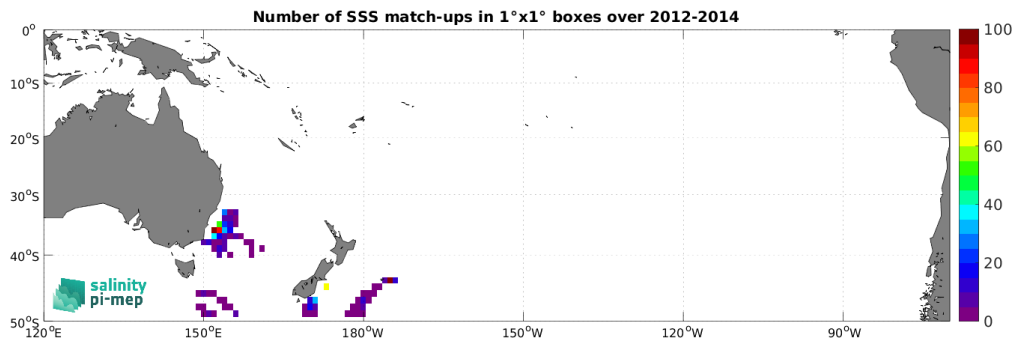
Figure 5: Number of SSS match-ups between Marine mammals SSS and the Aquarius SSS L3 OR v5 - Monthly - Rain mask (NASA-GSFC) SSS product for the South Pacific Ocean Pi-MEP region over 1^\circ \times 1^\circ boxes and for the full satellite product period.
