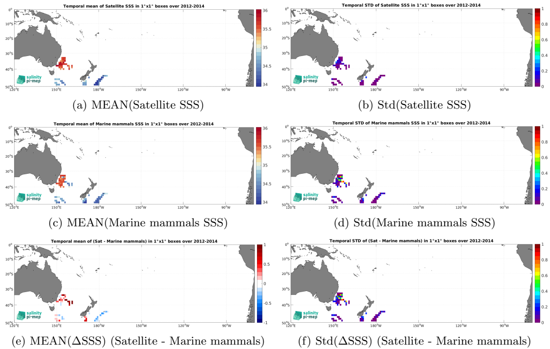
Figure 6: Temporal mean (left) and Std (right) of SSS from Aquarius SSS L3 OR v5 - Monthly - Rain mask (NASA-GSFC) (top), Marine mammals (middle), and of \Delta SSS (Satellite - Marine mammals). Only match-up pairs are used to generate these maps.
