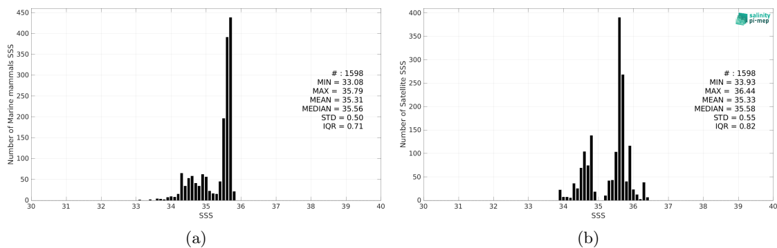
Figure 2: Histograms of SSS from Marine mammals (a) and Aquarius SSS L3 OR v5 - Monthly - Rain mask (NASA-GSFC) (b) considering all match-up pairs per bins of 0.1 over the South Pacific Ocean Pi-MEP region and for the full satellite product period.
