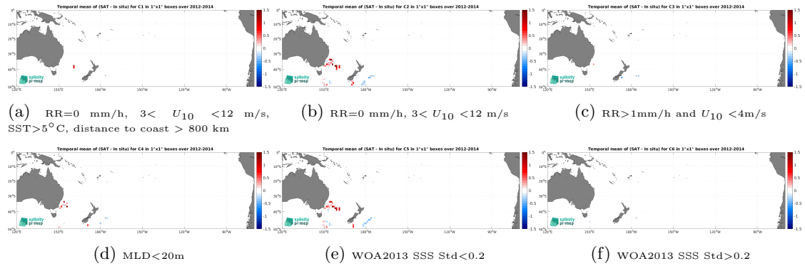
Figure 12: Temporal mean gridded over spatial boxes of size 1^{\circ}\times 1^{\circ} of \Delta\text{SSS} (Aquarius SSS L3 OR v5 - Monthly - Rain mask (NASA-GSFC) - Marine mammals) for 6 different subdatasets corresponding to:RR=0 mm/h, 3 < U_{10} < 12 m/s, SST >5^{\circ}\text{C} , distance to coast > 800 km (a), RR=0 mm/h, 3 < U_{10} < 12 m/s (b), RR >1 mm/h and U_{10} < 4 m/s (c),MLD <20 m (d),WOA2013 SSS Std <0.2 (e),WOA2013 SSS Std >0.2 (f).
