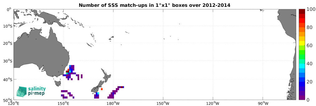
Figure 4: Number of SSS match-ups between Marine mammals SSS and the Aquarius SSS L3 OR v5 - Monthly - Rain mask (NASA-GSFC) SSS product for the South Pacific Ocean Pi-MEP region over 1^\circ \times 1^\circ boxes and for the full satellite product period.
