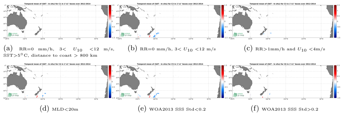
Figure 12: Temporal mean gridded over spatial boxes of size 1^\circ \times 1^\circ of \Delta SSS (Aquarius-L3-OR-V5-MONTHLY-RAIN-MASK-1DEG - Sea mammals) for 6 different subdatasets corresponding to: RR=0 mm/h, 3 < U_{10} < 12 m/s, SST > 5^\circ C , distance to coast > 800 km (a), RR=0 mm/h, 3 < U_{10} < 12 m/s (b), RR > 1 mm/h and U_{10} < 4 m/s (c), MLD < 20 m (d), WOA2013 SSS Std < 0.2 (e), WOA2013 SSS Std > 0.2 (f).
