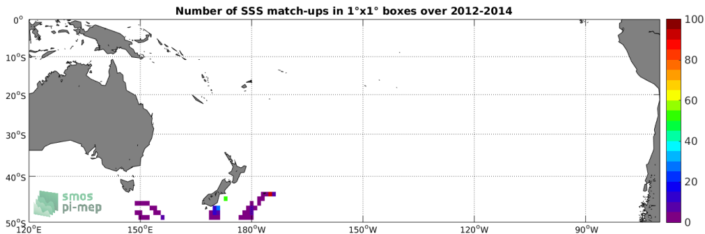
Figure 4: Number of SSS match-ups between Sea mammals SSS and the Aquarius-L3-OR-V5-MONTHLY-RAIN-MASK-1DEG SSS product for the South Pacific Ocean Pi-MEP region over 1°x1° boxes and for the full satellite product period.
