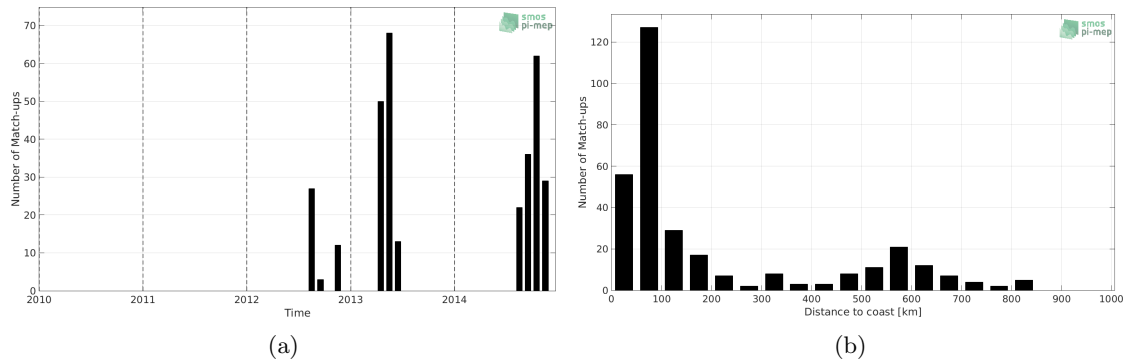
Figure 1: Number of match-ups between Sea mammals and Aquarius-L3-OR-V5-MONTHLY-RAIN-MASK-1DEG SSS as a function of time (a) and as function of the distance to coast (b) over the South Pacific Ocean Pi-MEP region and for the full satellite product period.
