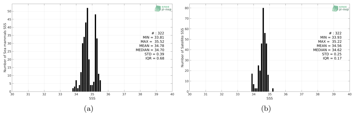
Figure 2: Histograms of SSS from Sea mammals (a) and Aquarius-L3-OR-V5-MONTHLY-RAIN-MASK-1DEG (b) considering all match-up pairs per bins of 0.1 over the South Pacific Ocean Pi-MEP region and for the full satellite product period.
