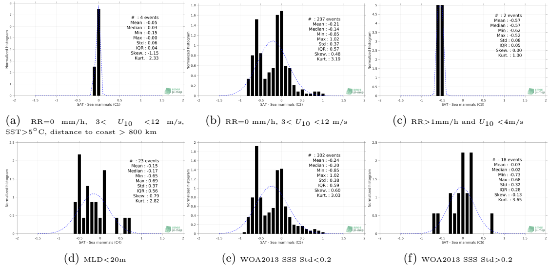
Figure 13: Normalized histogram of \Delta\text{SSS} (Aquarius-L3-OR-V5-MONTHLY-RAIN-MASK-1DEG - Sea mammals) for 6 different subdatasets corresponding to: RR=0 mm/h, 3 < U_{10} < 12 m/s, SST>5°C, distance to coast > 800 km (a), RR=0 mm/h, 3 < U_{10} < 12 m/s (b), RR>1mm/h and U_{10} < 4 m/s (c), MLD<20m (d), WOA2013 SSS Std<0.2 (e), WOA2013 SSS Std>0.2 (f).
