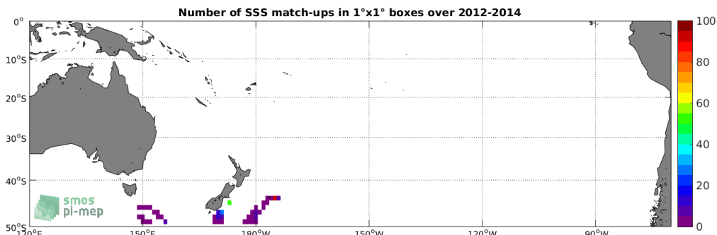
Figure 4: Number of SSS match-ups between Sea mammals SSS and the Aquarius-L3-OR-V5-MONTHLY-RAIN-MASK-1DEG SSS product for the South Pacific Ocean Pi-MEP region over 1^\circ \times 1^\circ boxes and for the full satellite product period.
