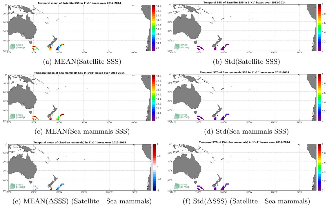
Figure 6: Temporal mean (left) and Std (right) of SSS from Aquarius-L3-OR-V5-MONTHLY-RAIN-MASK-1DEG (top), Sea mammals (middle), and of \Delta SSS (Satellite - Sea mammals). Only match-up pairs are used to generate these maps.
