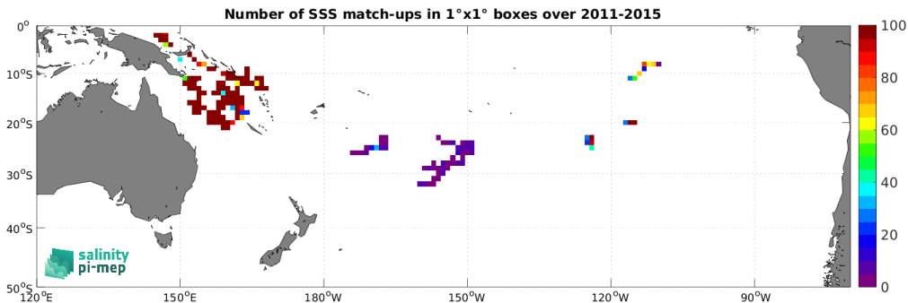
Figure 4: Number of SSS match-ups between Surface drifters SSS and the Aquarius SSS L3 OR v5 - Monthly - Rain mask (NASA-GSFC) SSS product for the South Pacific Ocean Pi-MEP region over 1^\circ \times 1^\circ boxes and for the full satellite product period.
