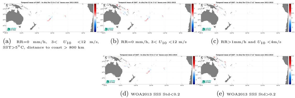
Figure 13: Temporal mean gridded over spatial boxes of size 1^\circ \times 1^\circ of \Delta SSS (Aquarius SSS L3 OR v5 - Monthly - Rain mask (NASA-GSFC) - Surface drifters) for 5 different subdatasets corresponding to:RR=0 mm/h, 3 < U_{10} < 12 m/s, SST >5^\circ\text{C} , distance to coast > 800 km (a), RR=0 mm/h, 3 < U_{10} < 12 m/s (b), RR >1 mm/h and U_{10} < 4 m/s (c), WOA2013 SSS Std <0.2 (d), WOA2013 SSS Std >0.2 (e).
