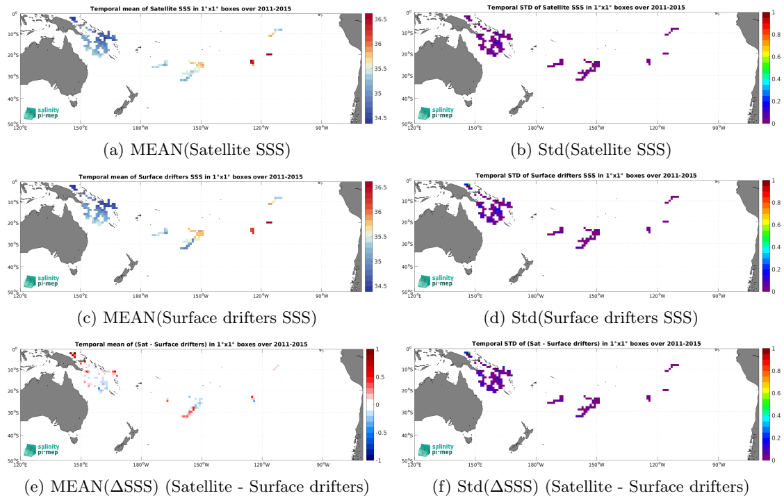
Figure 6: Temporal mean (left) and Std (right) of SSS from Aquarius SSS L3 OR v5 - Monthly - Rain mask (NASA-GSFC) (top), Surface drifters (middle), and of \Delta SSS (Satellite - Surface drifters). Only match-up pairs are used to generate these maps.
