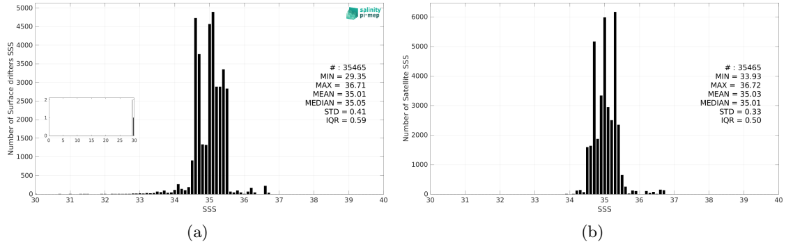
Figure 3: Histograms of SSS from Surface drifters (a) and Aquarius SSS L3 OR v5 - Monthly - Rain mask (NASA-GSFC) (b) considering all match-up pairs per bins of 0.1 over the South Pacific Ocean Pi-MEP region and for the full satellite product period.
