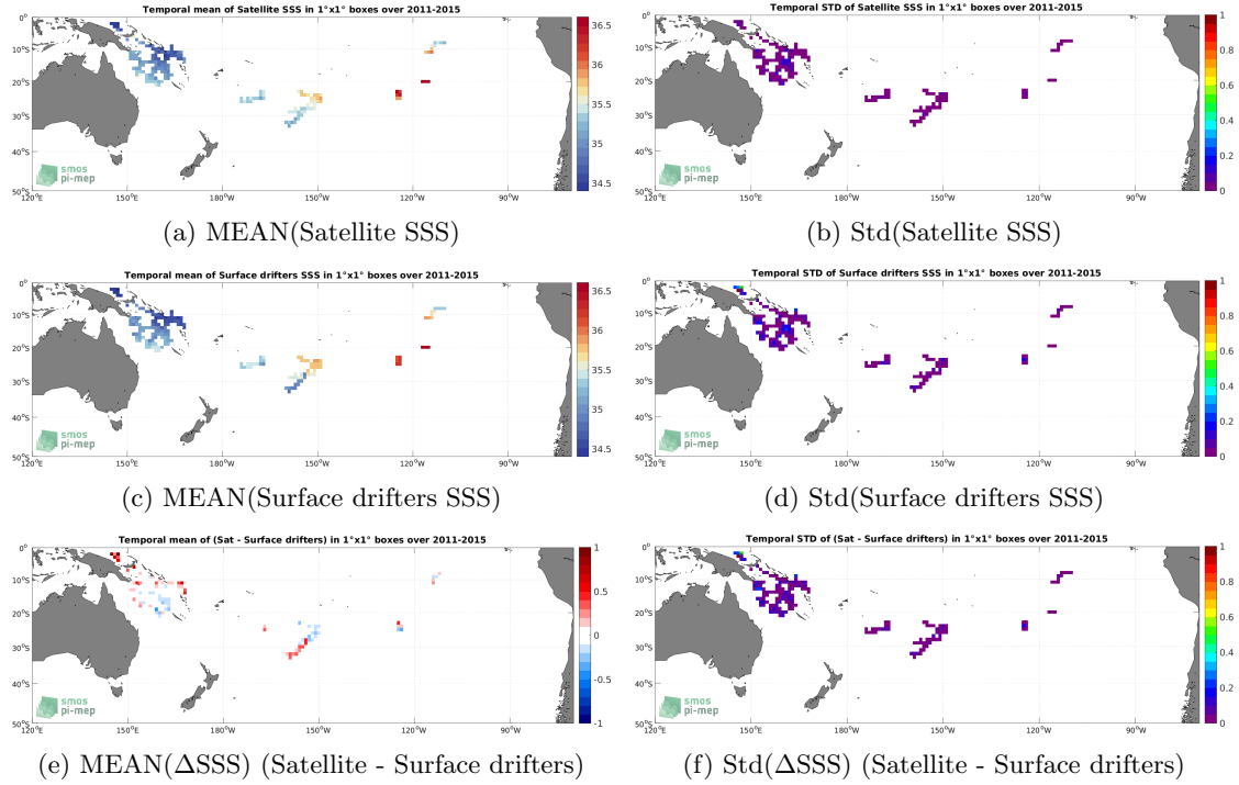
Figure 5: Temporal mean (left) and Std (right) of SSS from Aquarius SSS L3 OR v5 - Monthly - Rain mask (NASA-GSFC) (top), Surface drifters (middle), and of \Delta SSS (Satellite - Surface drifters). Only match-up pairs are used to generate these maps.
