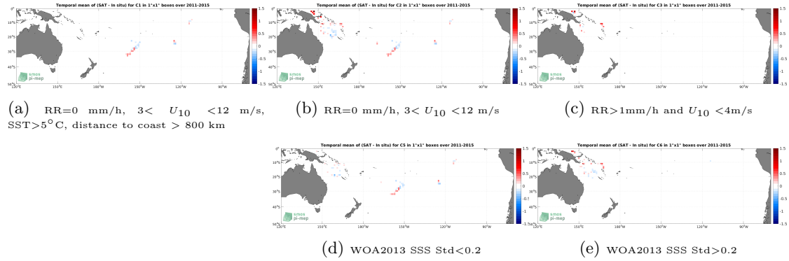
Figure 11: Temporal mean gridded over spatial boxes of size 1^{\circ}\times 1^{\circ} of \Delta\text{SSS} (Aquarius SSS L3 OR v5 - Monthly - Rain mask (NASA-GSFC) - Surface drifters) for 5 different subdatasets corresponding to:RR=0 mm/h, 3 < U_{10} < 12 m/s, SST > 5^{\circ}\text{C} , distance to coast > 800 km (a), RR=0 mm/h, 3 < U_{10} < 12 m/s (b), RR > 1 mm/h and U_{10} < 4 m/s (c), WOA2013 SSS Std < 0.2 (d), WOA2013 SSS Std > 0.2 (e).
