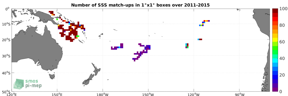
Figure 3: Number of SSS match-ups between Surface drifters SSS and the Aquarius SSS L3 OR v5 - Monthly - Rain mask (NASA-GSFC) SSS product for the South Pacific Ocean Pi-MEP region over 1^\circ \times 1^\circ boxes and for the full satellite product period.
