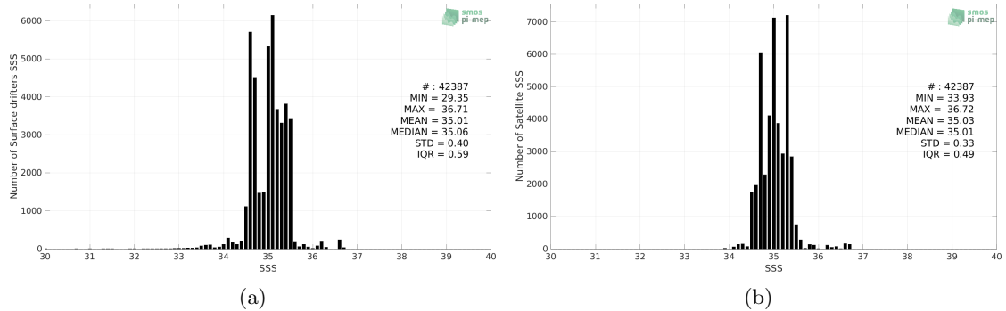
Figure 2: Histograms of SSS from Surface drifters (a) and Aquarius SSS L3 OR v5 - Monthly - Rain mask (NASA-GSFC) (b) considering all match-up pairs per bins of 0.1 over the South Pacific Ocean Pi-MEP region and for the full satellite product period.
