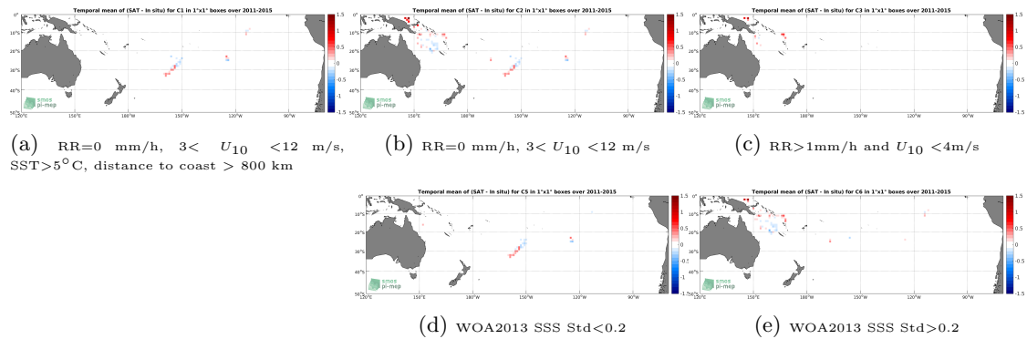
Figure 11: Temporal mean gridded over spatial boxes of size 1^\circ \times 1^\circ of \Delta SSS (Aquarius-L3-OR-V5-MONTHLY-RAIN-MASK-1DEG - Surface drifters) for 5 different subdatasets corresponding to:RR=0 mm/h, 3 < U_{10} < 12 m/s, SST >5^\circ C, distance to coast > 800 km (a), RR=0 mm/h, 3 < U_{10} < 12 m/s (b), RR >1 mm/h and U_{10} < 4 m/s (c), WOA2013 SSS Std <0.2 (d), WOA2013 SSS Std >0.2 (e).
