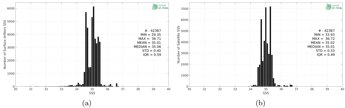
Figure 2: Histograms of SSS from Surface drifters (a) and Aquarius-L3-OR-V5-MONTHLY-RAIN-MASK-1DEG (b) considering all match-up pairs per bins of 0.1 over the South Pacific Ocean Pi-MEP region and for the full satellite product period.
