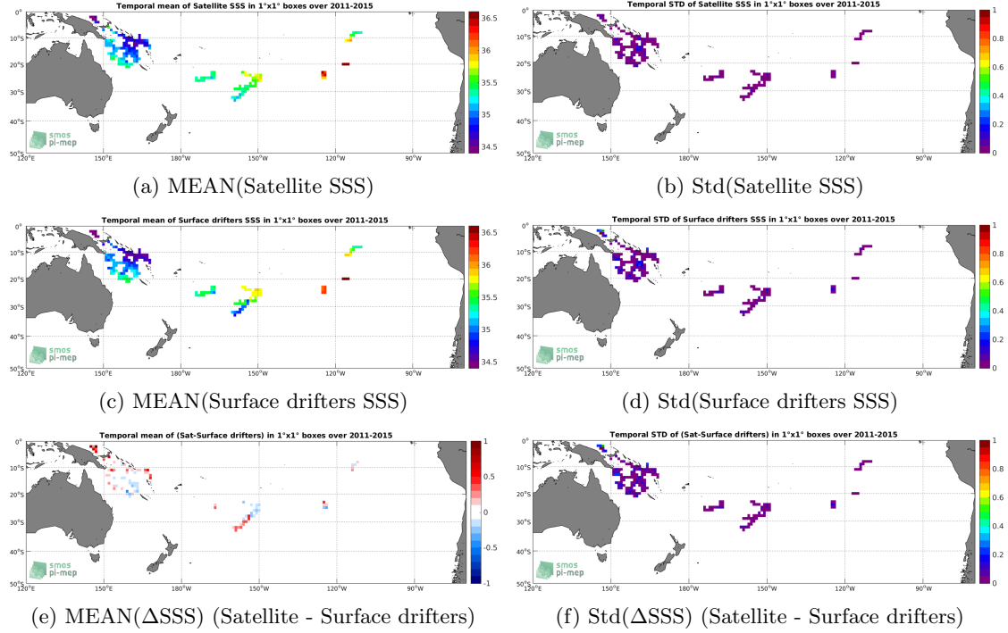
Figure 5: Temporal mean (left) and Std (right) of SSS from Aquarius-L3-OR-V5-MONTHLY-RAIN-MASK-1DEG (top), Surface drifters (middle), and of \Delta SSS (Satellite - Surface drifters). Only match-up pairs are used to generate these maps.
