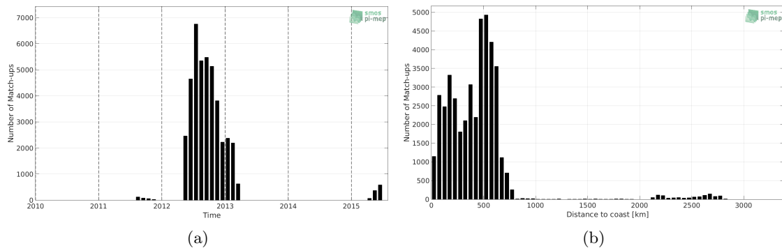
Figure 1: Number of match-ups between Surface drifters and Aquarius-L3-OR-V5-MONTHLY-RAIN-MASK-1DEG SSS as a function of time (a) and as function of the distance to coast (b) over the South Pacific Ocean Pi-MEP region and for the full satellite product period.
