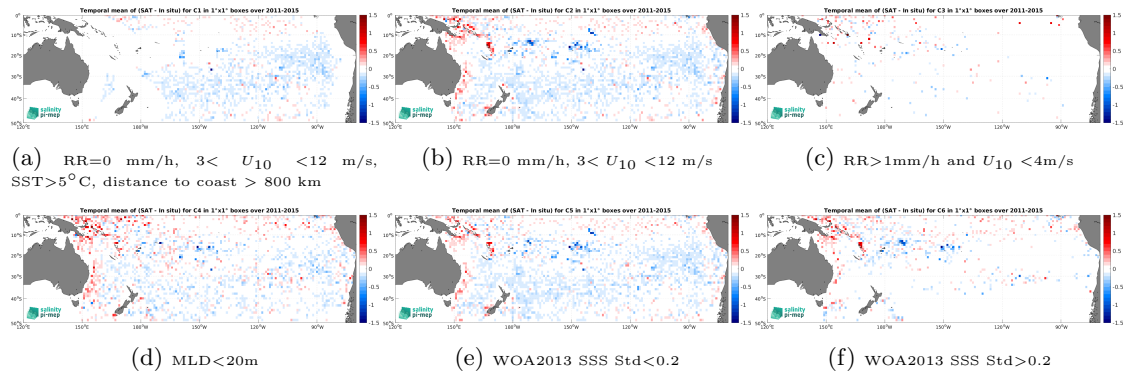
Figure 14: Temporal mean gridded over spatial boxes of size 1^\circ \times 1^\circ of \Delta SSS (Aquarius SSS L3 OR v5 - Monthly - Rain mask (NASA-GSFC) - Argo) for 6 different subdatasets corresponding to:RR=0 mm/h, 3 < U_{10} < 12 m/s, SST>5°C, distance to coast > 800 km (a), RR=0 mm/h, 3 < U_{10} < 12 m/s (b), RR>1mm/h and U_{10} < 4 m/s (c),MLD<20m (d),WOA2013 SSS Std<0.2 (e),WOA2013 SSS Std>0.2 (f).
