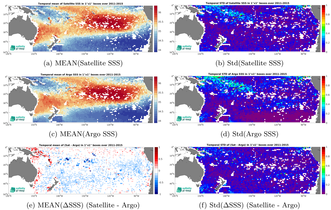
Figure 7: Temporal mean (left) and Std (right) of SSS from Aquarius SSS L3 OR v5 - Monthly - Rain mask (NASA-GSFC) (top), Argo (middle), and of \Delta SSS (Satellite - Argo). Only match-up pairs are used to generate these maps.
