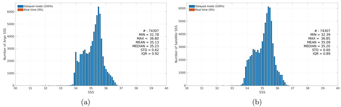
Figure 3: Histograms of SSS from Argo (a) and Aquarius SSS L3 OR v5 - Monthly - Rain mask (NASA-GSFC) (b) considering all match-up pairs per bins of 0.1 over the South Pacific Ocean Pi-MEP region and for the full satellite product period.
