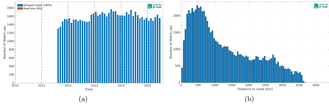
Figure 2: Number of match-ups between Argo and Aquarius SSS L3 OR v5 - Monthly - Rain mask (NASA-GSFC) SSS as a function of time (a) and as function of the distance to coast (b) over the South Pacific Ocean Pi-MEP region and for the full satellite product period.
