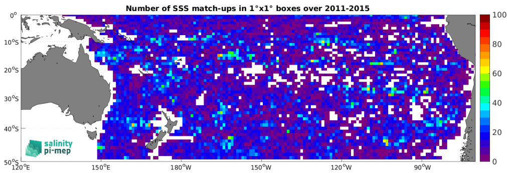
Figure 5: Number of SSS match-ups between Argo SSS and the Aquarius SSS L3 OR v5 - Monthly - Rain mask (NASA-GSFC) SSS product for the South Pacific Ocean Pi-MEP region over 1^\circ \times 1^\circ boxes and for the full satellite product period.
