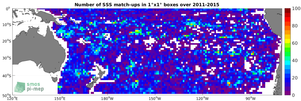
Figure 4: Number of SSS match-ups between Argo SSS and the Aquarius SSS L3 OR v5 - Monthly - Rain mask (NASA-GSFC) SSS product for the South Pacific Ocean Pi-MEP region over 1^\circ \times 1^\circ boxes and for the full satellite product period.
