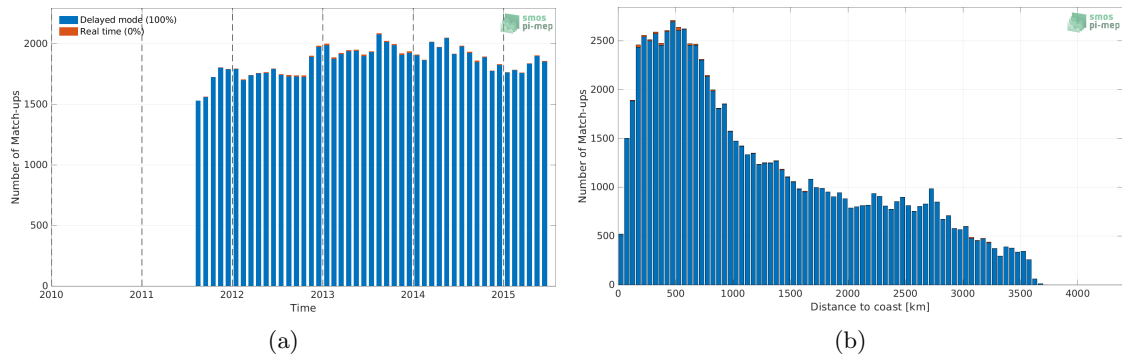
Figure 1: Number of match-ups between Argo and Aquarius SSS L3 OR v5 - Monthly - Rain mask (NASA-GSFC) SSS as a function of time (a) and as function of the distance to coast (b) over the South Pacific Ocean Pi-MEP region and for the full satellite product period.
