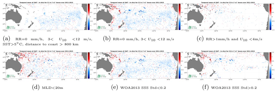
Figure 12: Temporal mean gridded over spatial boxes of size 1^\circ \times 1^\circ of \Delta SSS (Aquarius SSS L3 OR v5 - Monthly - Rain mask (NASA-GSFC) - Argo) for 6 different subdatasets corresponding to:RR=0 mm/h, 3 < U_{10} < 12 m/s, SST >5^\circ C, distance to coast > 800 km (a), RR=0 mm/h, 3 < U_{10} < 12 m/s (b), RR >1 mm/h and U_{10} < 4 m/s (c),MLD <20 m (d),WOA2013 SSS Std <0.2 (e),WOA2013 SSS Std >0.2 (f).
