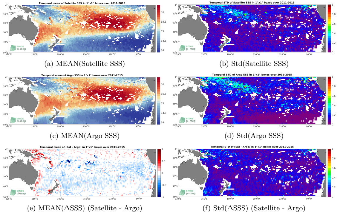
Figure 6: Temporal mean (left) and Std (right) of SSS from Aquarius SSS L3 OR v5 - Monthly - Rain mask (NASA-GSFC) (top), Argo (middle), and of \Delta SSS (Satellite - Argo). Only match-up pairs are used to generate these maps.
