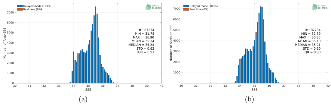
Figure 2: Histograms of SSS from Argo (a) and Aquarius SSS L3 OR v5 - Monthly - Rain mask (NASA-GSFC) (b) considering all match-up pairs per bins of 0.1 over the South Pacific Ocean Pi-MEP region and for the full satellite product period.
