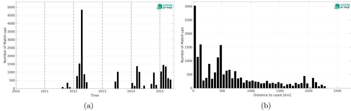
Figure 2: Number of match-ups between TSG (SAMOS) and Aquarius SSS L3 CAP v5 - 7-Day running (JPL) SSS as a function of time (a) and as function of the distance to coast (b) over the South Pacific Ocean Pi-MEP region and for the full satellite product period.
