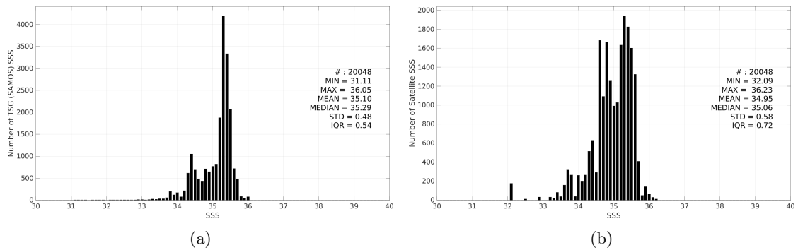
Figure 3: Histograms of SSS from TSG (SAMOS) (a) and Aquarius SSS L3 CAP v5 - 7-Day running (JPL) (b) considering all match-up pairs per bins of 0.1 over the South Pacific Ocean Pi-MEP region and for the full satellite product period.
