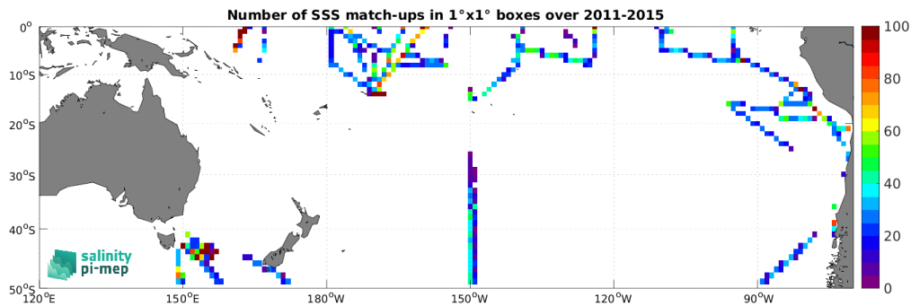
Figure 5: Number of SSS match-ups between TSG (SAMOS) SSS and the Aquarius SSS L3 CAP v5 - 7-Day running (JPL) SSS product for the South Pacific Ocean Pi-MEP region over 1^\circ \times 1^\circ boxes and for the full satellite product period.
