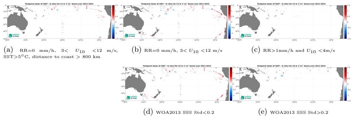
Figure 14: Temporal mean gridded over spatial boxes of size 1^\circ \times 1^\circ of \Delta\text{SSS} (Aquarius SSS L3 CAP v5 - 7-Day running (JPL) - TSG (SAMOS)) for 5 different subdatasets corresponding to:RR=0 mm/h, 3 < U_{10} < 12 m/s, SST>5°C, distance to coast > 800 km (a), RR=0 mm/h, 3 < U_{10} < 12 m/s (b), RR>1mm/h and U_{10} < 4 m/s (c), WOA2013 SSS Std<0.2 (d), WOA2013 SSS Std>0.2 (e).
