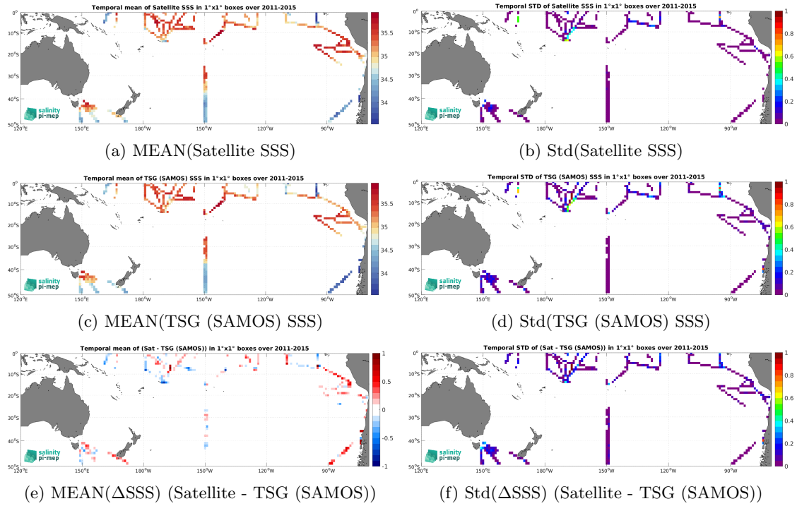
Figure 7: Temporal mean (left) and Std (right) of SSS from Aquarius SSS L3 CAP v5 - 7-Day running (JPL) (top), TSG (SAMOS) (middle), and of \Delta SSS (Satellite - TSG (SAMOS)). Only match-up pairs are used to generate these maps.
