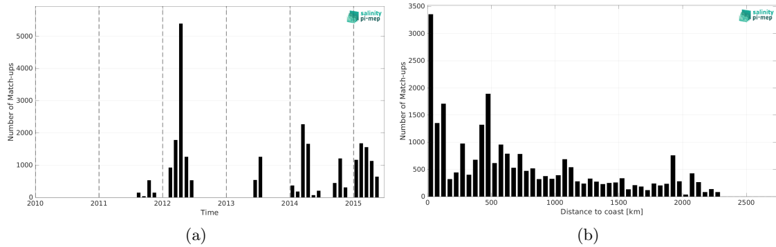
Figure 1: Number of match-ups between TSG (SAMOS) and Aquarius SSS L3 CAP v5 - 7-Day running (JPL) SSS as a function of time (a) and as function of the distance to coast (b) over the South Pacific Ocean Pi-MEP region and for the full satellite product period.
