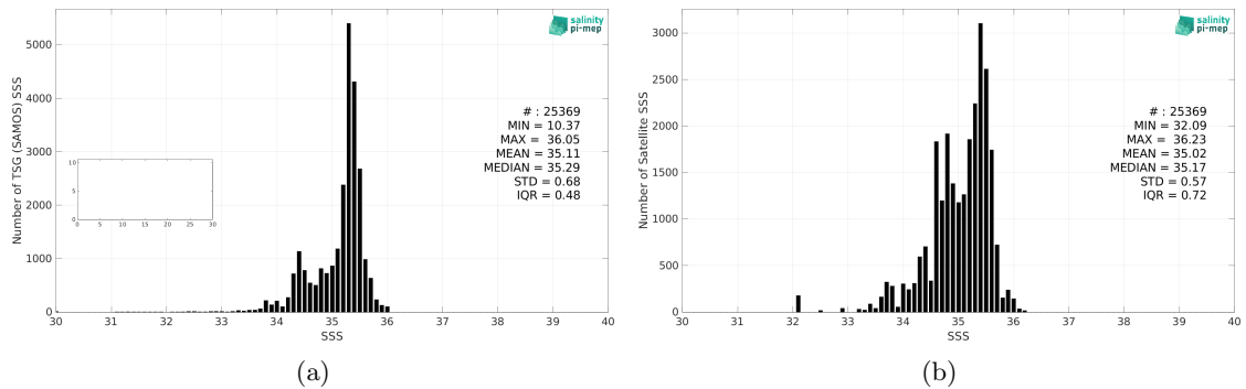
Figure 2: Histograms of SSS from TSG (SAMOS) (a) and Aquarius SSS L3 CAP v5 - 7-Day running (JPL) (b) considering all match-up pairs per bins of 0.1 over the South Pacific Ocean Pi-MEP region and for the full satellite product period.
