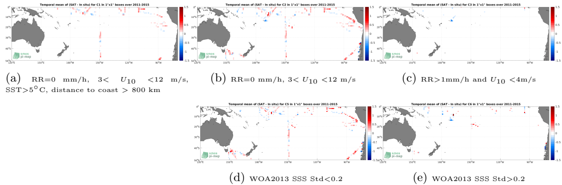
Figure 12: Temporal mean gridded over spatial boxes of size 1^\circ \times 1^\circ of \Delta\text{SSS} (Aquarius SSS L3 CAP v5 - 7-Day running (JPL) - TSG (SAMOS)) for 5 different subdatasets corresponding to:RR=0 mm/h, 3 < U_{10} < 12 m/s, SST >5^\circ\text{C} , distance to coast > 800 km (a), RR=0 mm/h, 3 < U_{10} < 12 m/s (b), RR >1 mm/h and U_{10} < 4 m/s (c), WOA2013 SSS Std <0.2 (d), WOA2013 SSS Std >0.2 (e).
