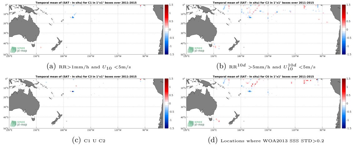
Figure 12: Temporal mean gridded over spatial boxes of size 1^\circ \times 1^\circ of \Delta SSS (Aquarius-L3-JPL-V5-7DAY-RUNNING - TSG-SAMOS) for 4 different subdatasets corresponding to: RR > 1\text{mm/h} and U_{10} < 5\text{m/s} (a), RR^{10d} > 5\text{mm/h} and U_{10}^{10d} < 5\text{m/s} (b), C1 U C2 (c), Locations where WOA2013 SSS STD > 0.2 (d).
