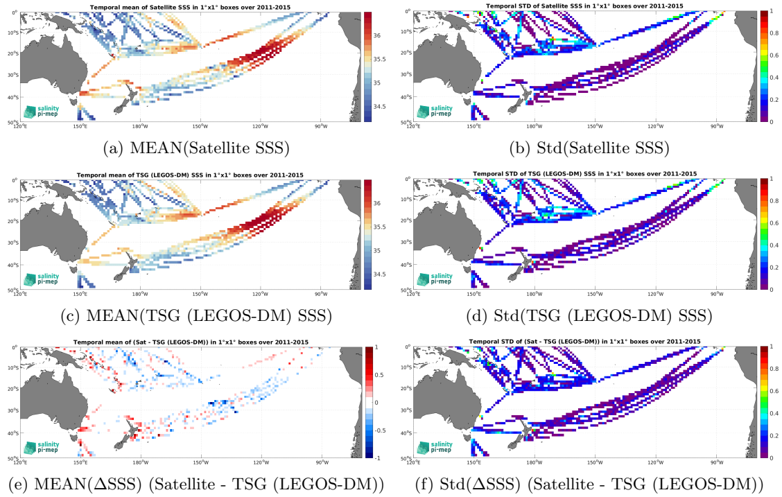
Figure 7: Temporal mean (left) and Std (right) of SSS from Aquarius SSS L3 CAP v5 - 7-Day running (JPL) (top), TSG (LEGOS-DM) (middle), and of \Delta SSS (Satellite - TSG (LEGOS-DM)). Only match-up pairs are used to generate these maps.
