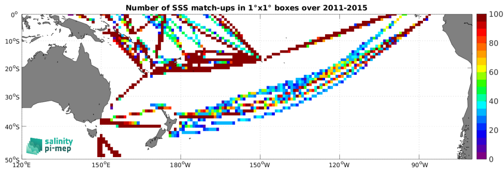
Figure 5: Number of SSS match-ups between TSG (LEGOS-DM) SSS and the Aquarius SSS L3 CAP v5 - 7-Day running (JPL) SSS product for the South Pacific Ocean Pi-MEP region over 1^\circ \times 1^\circ boxes and for the full satellite product period.
