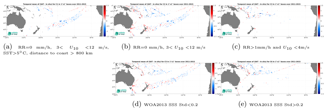
Figure 14: Temporal mean gridded over spatial boxes of size 1^\circ \times 1^\circ of \Delta\text{SSS} (Aquarius SSS L3 CAP v5 - 7-Day running (JPL) - TSG (LEGOS-DM)) for 5 different subdatasets corresponding to:RR=0 mm/h, 3 < U_{10} < 12 m/s, SST >5^\circ\text{C} , distance to coast > 800 km (a), RR=0 mm/h, 3 < U_{10} < 12 m/s (b), RR >1 mm/h and U_{10} < 4 m/s (c), WOA2013 SSS Std <0.2 (d), WOA2013 SSS Std >0.2 (e).
