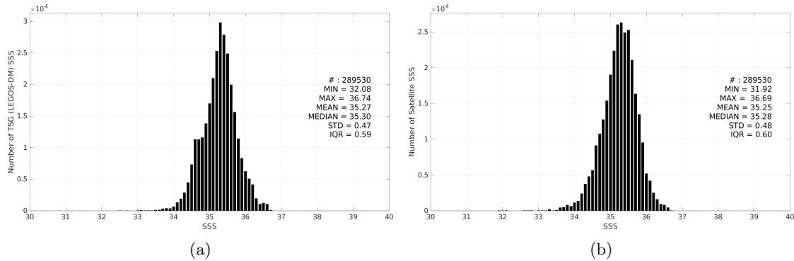
Figure 3: Histograms of SSS from TSG (LEGOS-DM) (a) and Aquarius SSS L3 CAP v5 - 7-Day running (JPL) (b) considering all match-up pairs per bins of 0.1 over the South Pacific Ocean Pi-MEP region and for the full satellite product period.
