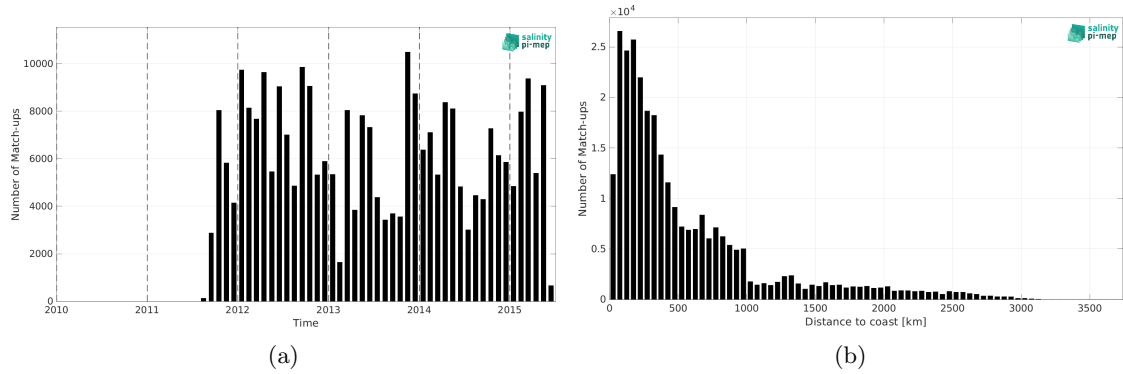
Figure 2: Number of match-ups between TSG (LEGOS-DM) and Aquarius SSS L3 CAP v5 - 7-Day running (JPL) SSS as a function of time (a) and as function of the distance to coast (b) over the South Pacific Ocean Pi-MEP region and for the full satellite product period.
