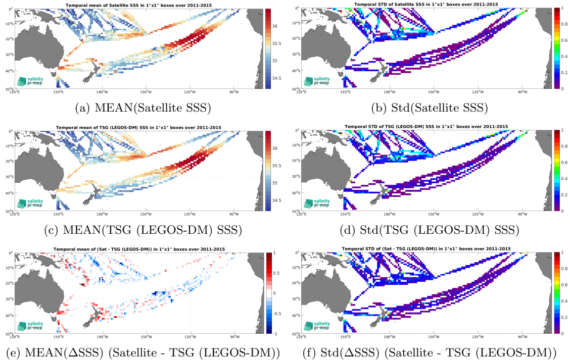
Figure 6: Temporal mean (left) and Std (right) of SSS from Aquarius SSS L3 CAP v5 - 7-Day running (JPL) (top), TSG (LEGOS-DM) (middle), and of \Delta SSS (Satellite - TSG (LEGOS-DM)). Only match-up pairs are used to generate these maps.
