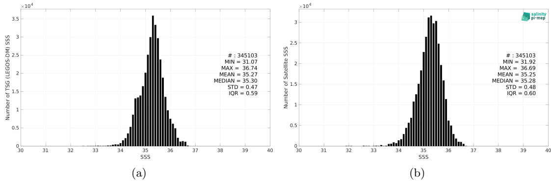
Figure 2: Histograms of SSS from TSG (LEGOS-DM) (a) and Aquarius SSS L3 CAP v5 - 7-Day running (JPL) (b) considering all match-up pairs per bins of 0.1 over the South Pacific Ocean Pi-MEP region and for the full satellite product period.
