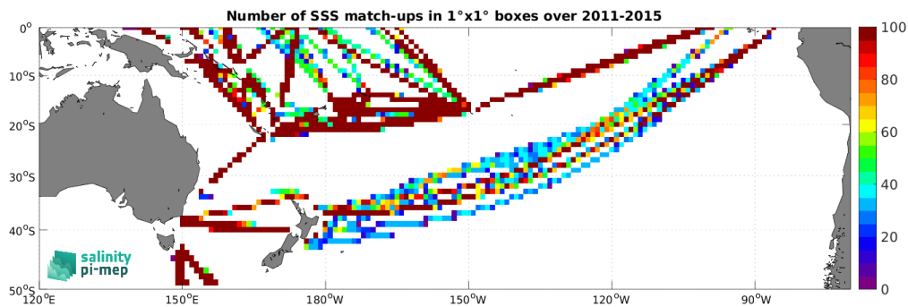
Figure 4: Number of SSS match-ups between TSG (LEGOS-DM) SSS and the Aquarius SSS L3 CAP v5 - 7-Day running (JPL) SSS product for the South Pacific Ocean Pi-MEP region over 1^\circ \times 1^\circ boxes and for the full satellite product period.
