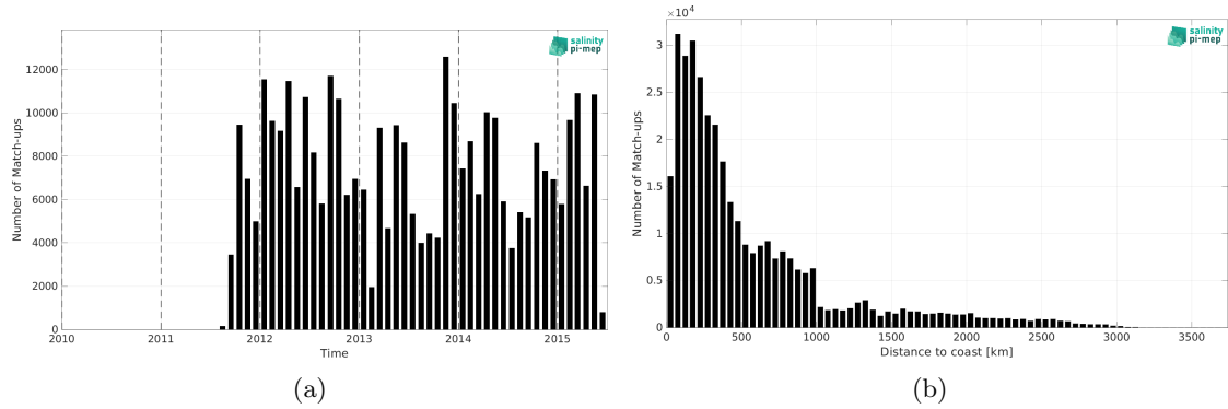
Figure 1: Number of match-ups between TSG (LEGOS-DM) and Aquarius SSS L3 CAP v5 - 7-Day running (JPL) SSS as a function of time (a) and as function of the distance to coast (b) over the South Pacific Ocean Pi-MEP region and for the full satellite product period.
