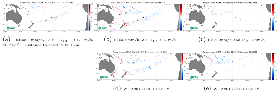
Figure 12: Temporal mean gridded over spatial boxes of size 1^\circ \times 1^\circ of \Delta SSS (Aquarius SSS L3 CAP v5 - 7-Day running (JPL) - TSG (LEGOS-DM)) for 5 different subdatasets corresponding to:RR=0 mm/h, 3 < U_{10} < 12 m/s, SST >5^\circ C, distance to coast > 800 km (a), RR=0 mm/h, 3 < U_{10} < 12 m/s (b), RR >1 mm/h and U_{10} < 4 m/s (c), WOA2013 SSS Std <0.2 (d), WOA2013 SSS Std >0.2 (e).
