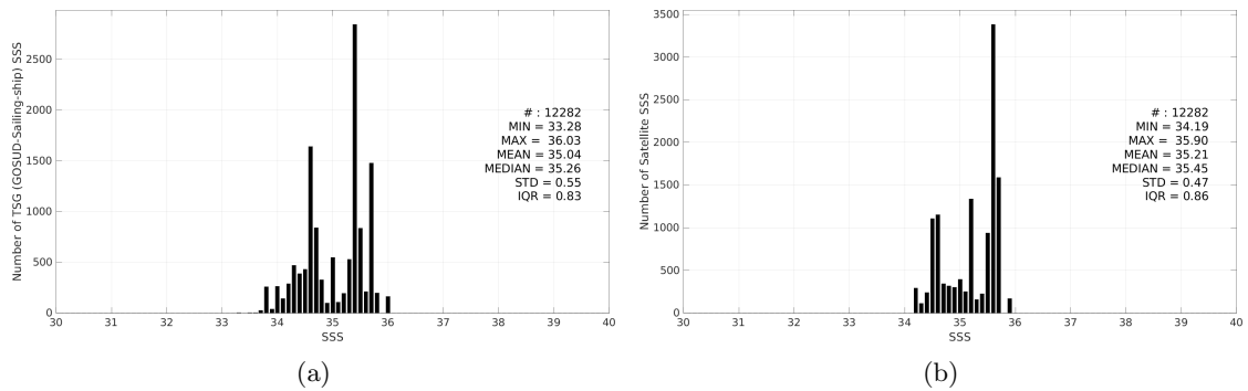
Figure 3: Histograms of SSS from TSG (GOSUD-Sailing-ship) (a) and Aquarius SSS L3 CAP v5 - 7-Day running (JPL) (b) considering all match-up pairs per bins of 0.1 over the South Pacific Ocean Pi-MEP region and for the full satellite product period.
