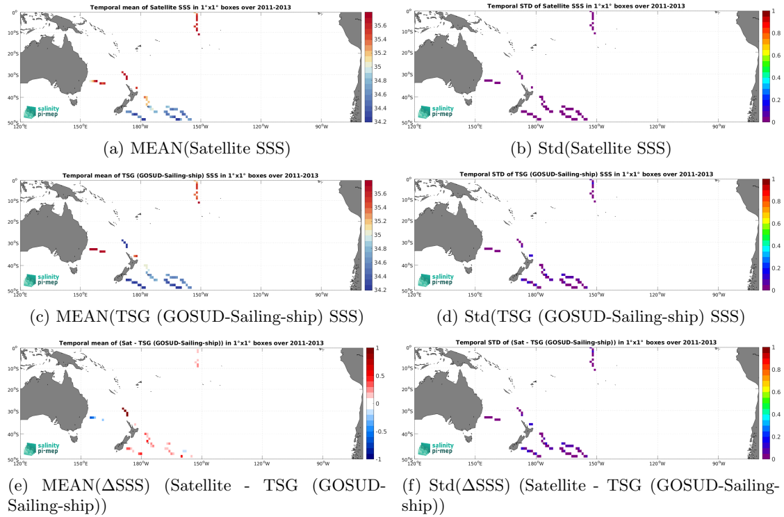
Figure 7: Temporal mean (left) and Std (right) of SSS from Aquarius SSS L3 CAP v5 - 7-Day running (JPL) (top), TSG (GOSUD-Sailing-ship) (middle), and of \Delta SSS (Satellite - TSG (GOSUD-Sailing-ship)). Only match-up pairs are used to generate these maps.
