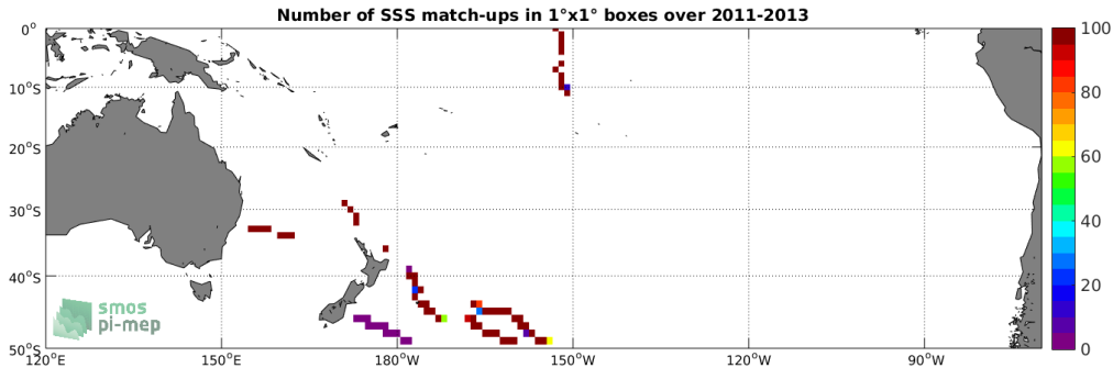
Figure 4: Number of SSS match-ups between TSG (GOSUD-Sailing-ship) SSS and the Aquarius SSS L3 CAP v5 - 7-Day running (JPL) SSS product for the South Pacific Ocean Pi-MEP region over 1^\circ \times 1^\circ boxes and for the full satellite product period.
