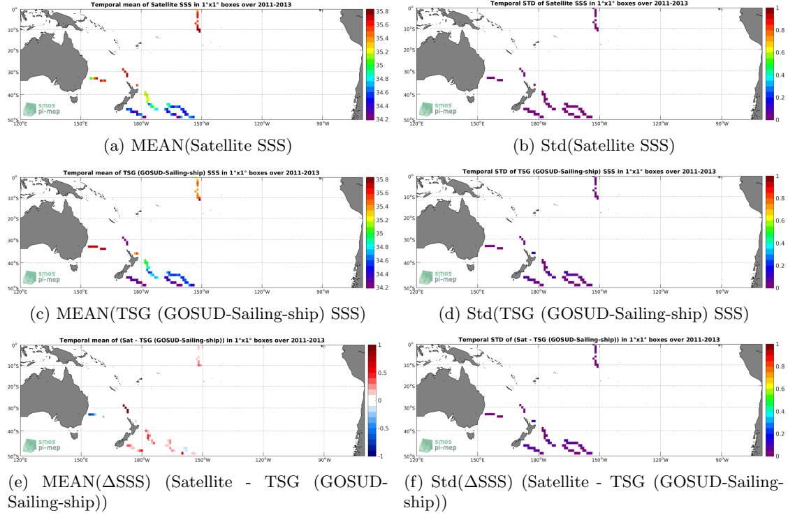
Figure 6: Temporal mean (left) and Std (right) of SSS from Aquarius SSS L3 CAP v5 - 7-Day running (JPL) (top), TSG (GOSUD-Sailing-ship) (middle), and of \Delta SSS (Satellite - TSG (GOSUD-Sailing-ship)). Only match-up pairs are used to generate these maps.
