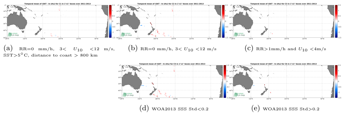
Figure 12: Temporal mean gridded over spatial boxes of size 1^\circ \times 1^\circ of \Delta\text{SSS} (Aquarius SSS L3 CAP v5 - 7-Day running (JPL) - TSG (GOSUD-Sailing-ship)) for 5 different subdatasets corresponding to:RR=0 mm/h, 3 < U_{10} < 12 m/s, SST>5°C, distance to coast > 800 km (a), RR=0 mm/h, 3 < U_{10} < 12 m/s (b), RR>1mm/h and U_{10} < 4 m/s (c), WOA2013 SSS Std<0.2 (d), WOA2013 SSS Std>0.2 (e).
