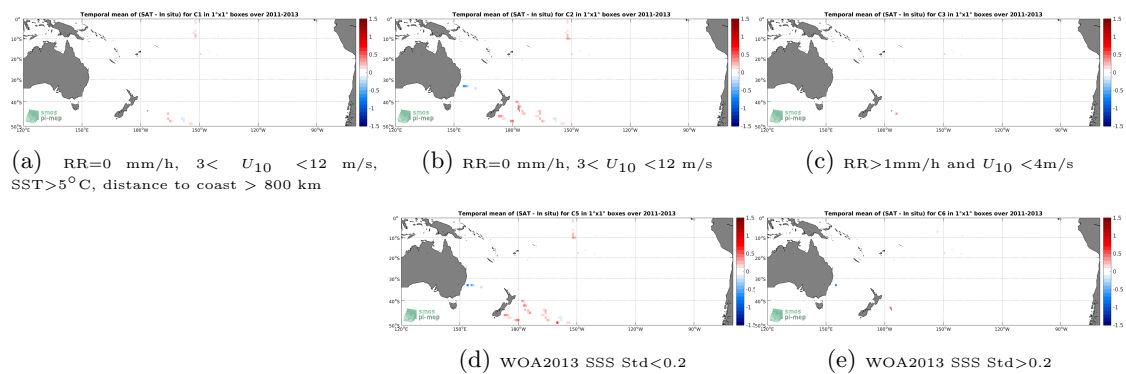
Figure 12: Temporal mean gridded over spatial boxes of size 1^\circ \times 1^\circ of \Delta SSS (Aquarius-L3-JPL-V5-7DAY-RUNNING - TSG-GOSUD-Sailing-ship) for 5 different subdatasets corresponding to: RR=0 mm/h, 3 < U_{10} < 12 m/s, SST > 5°C, distance to coast > 800 km (a), RR=0 mm/h, 3 < U_{10} < 12 m/s (b), RR > 1mm/h and U_{10} < 4 m/s (c), WOA2013 SSS Std < 0.2 (d), WOA2013 SSS Std > 0.2 (e).
